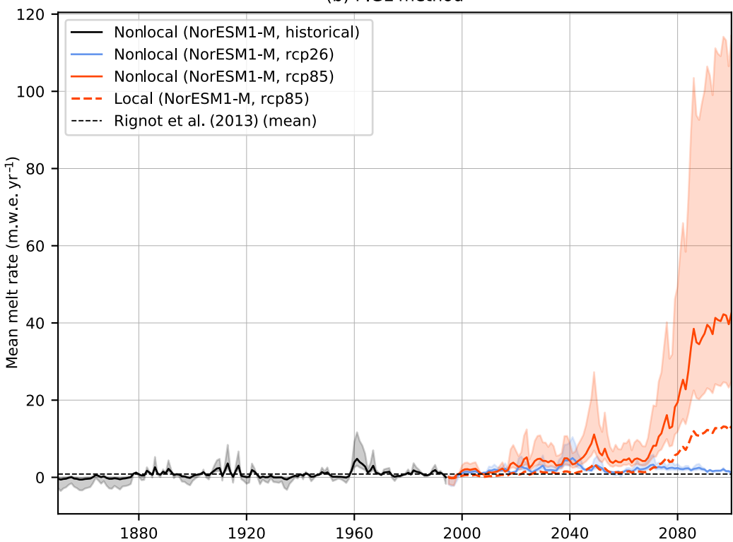
(b) PIGL method
