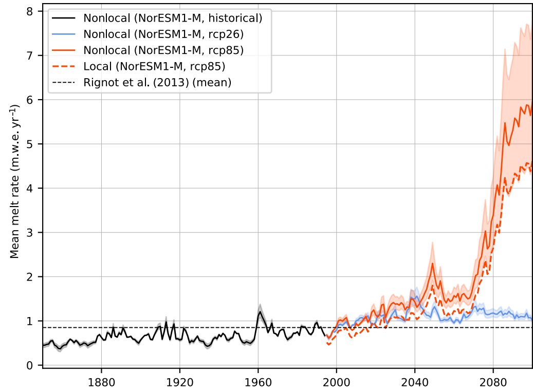
(a) MeanAnt method
