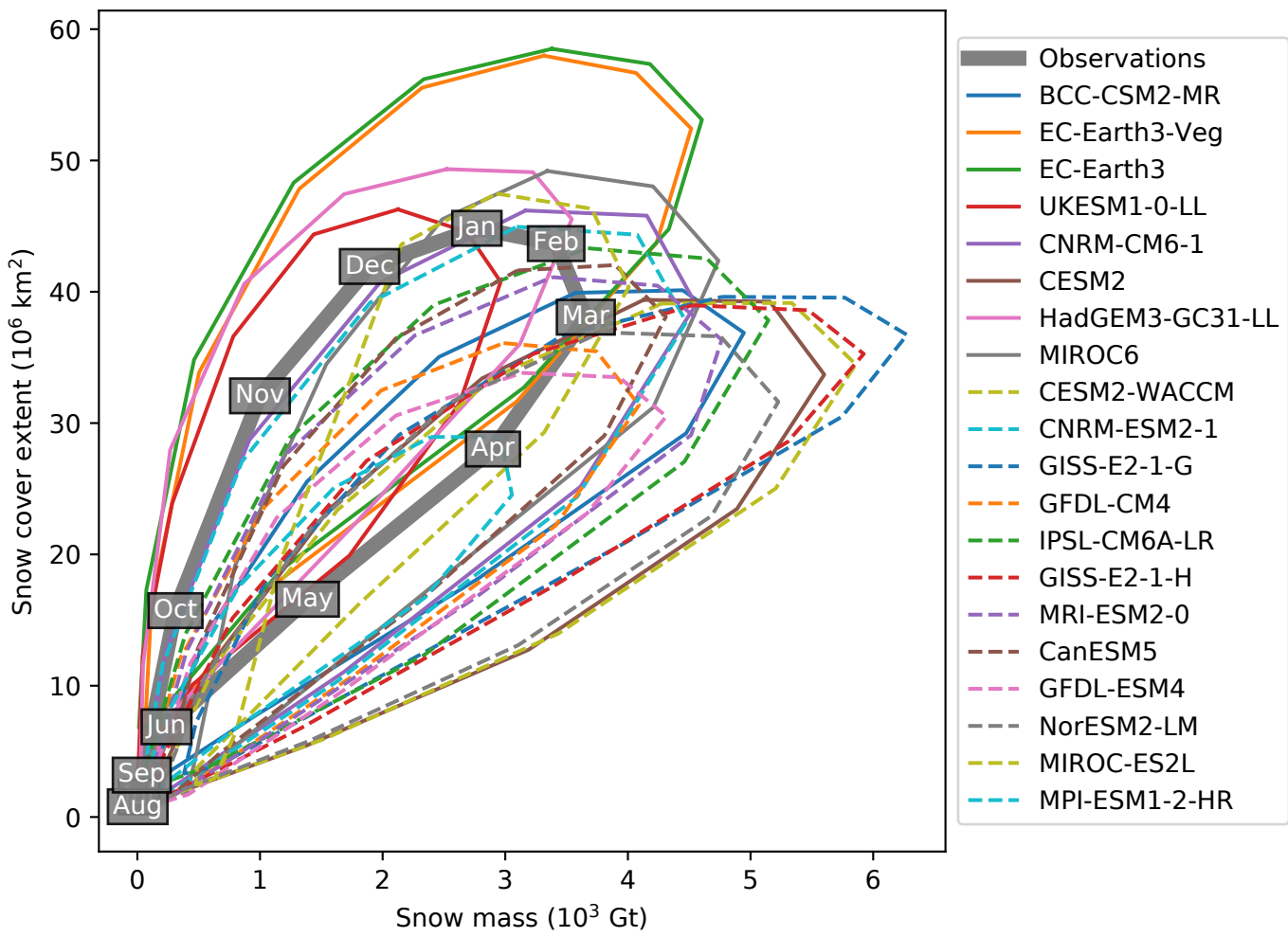
NH snow cover extent as a function of snow mass
