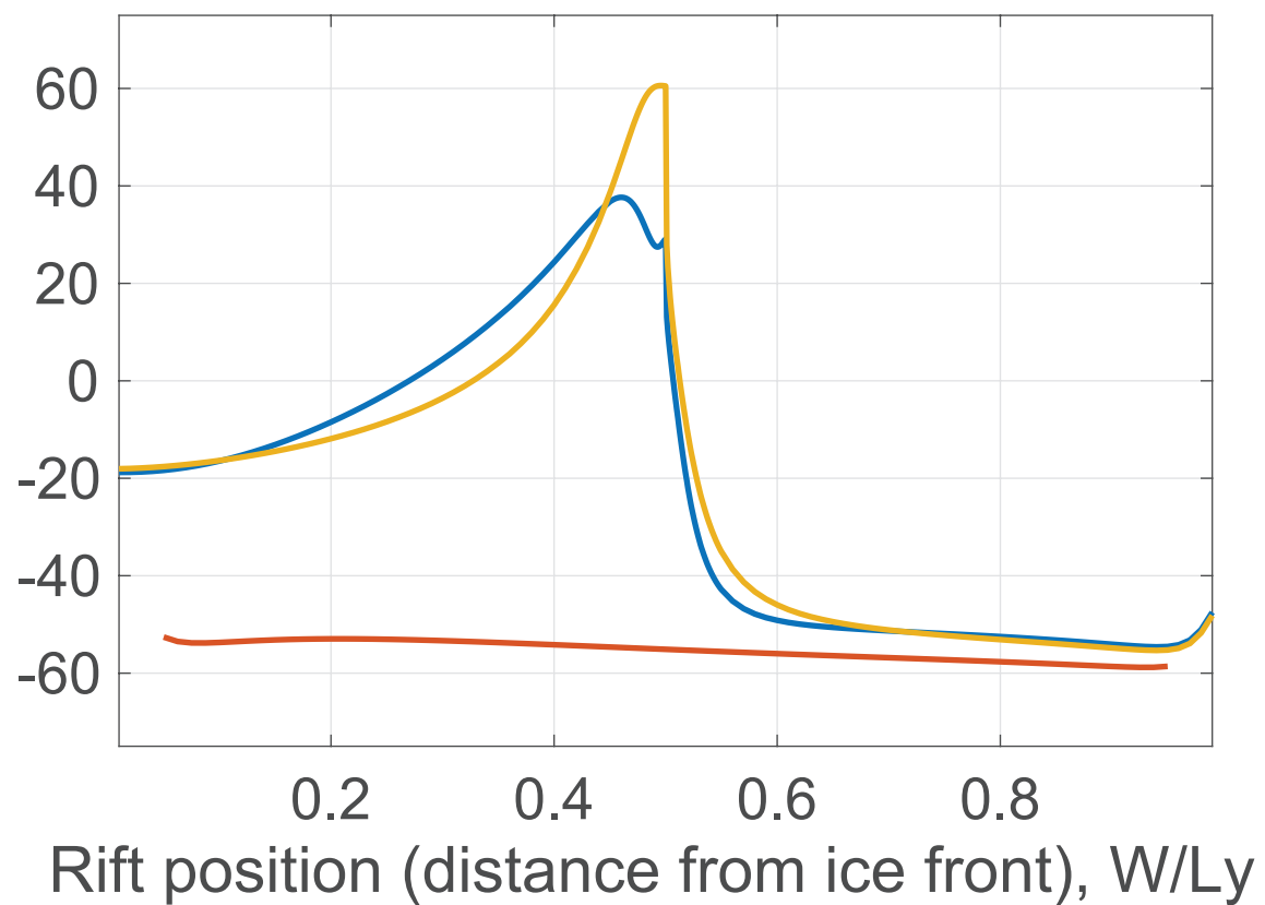
(a) Mode I stress intensity factor, K_I / K_{Ic}
