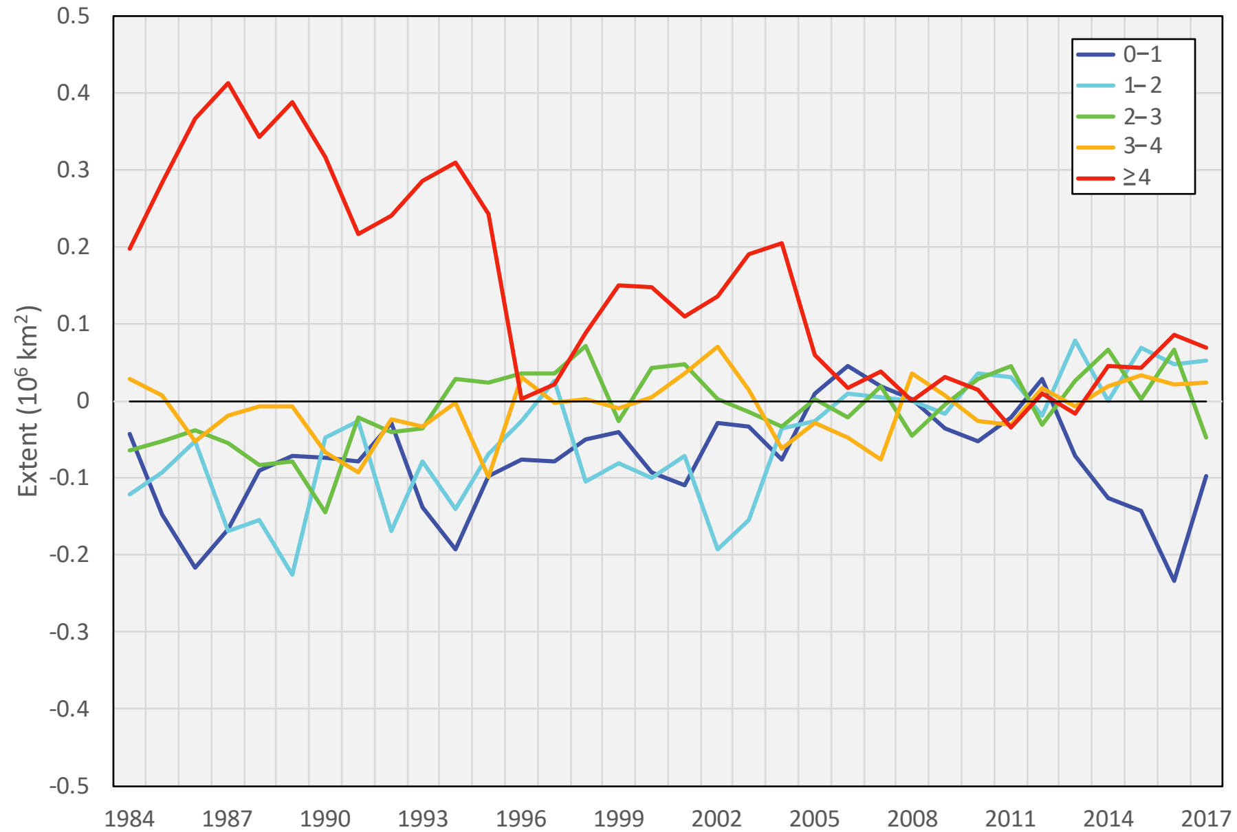
Late February age extent difference, Version 4 – Version 3
