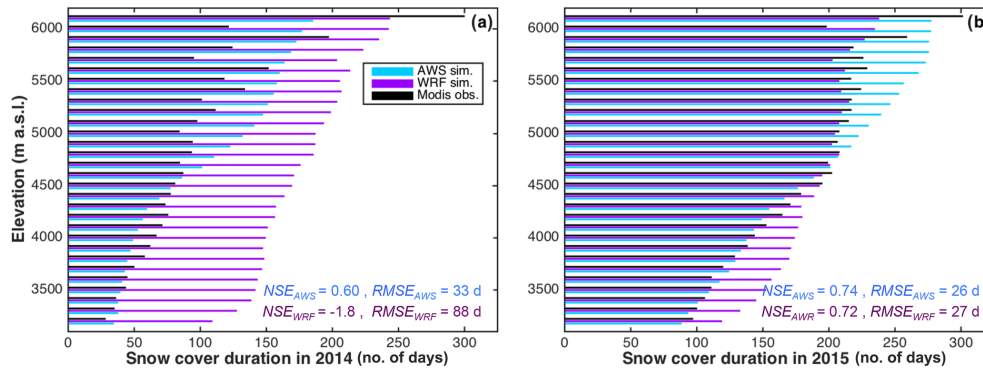
Figure 7. Snow cover duration per 200 m elevation band, from MODIS images (black), AWS forcing (blue) and WRF forcing (purple) for (a) 2014 and (b) 2015.
