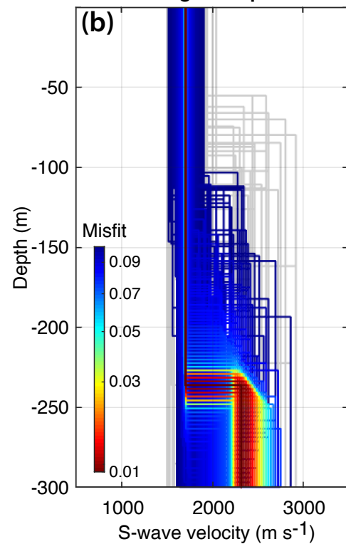
Inverted ground profiles
