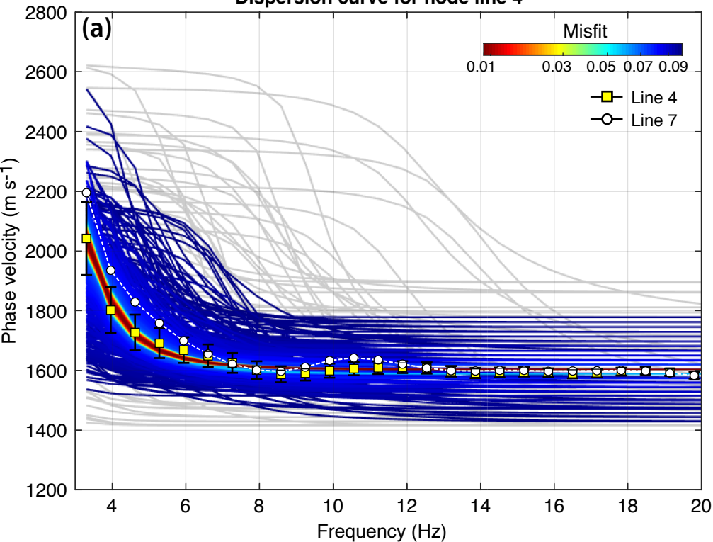
Dispersion curve for node line 4
