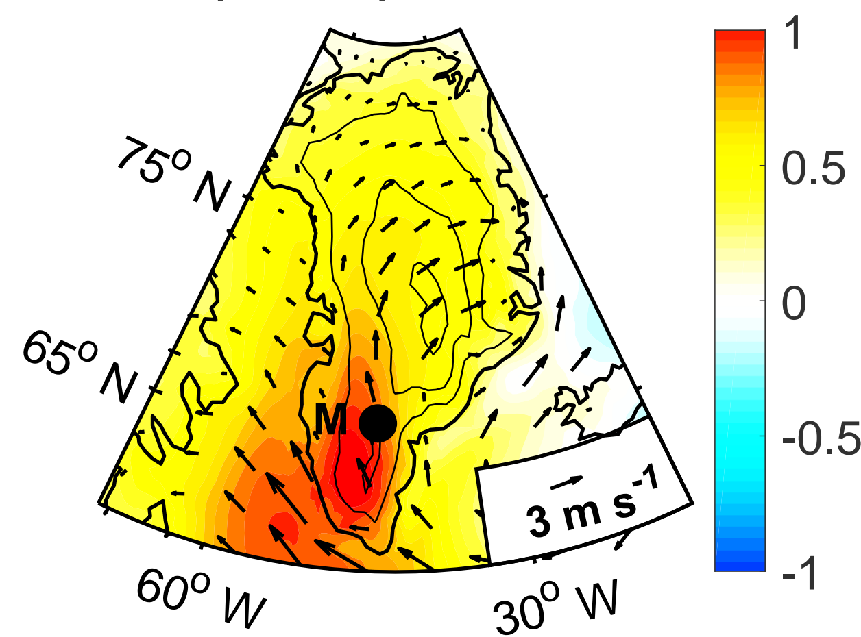
(e) T (norm.) and wind an.
