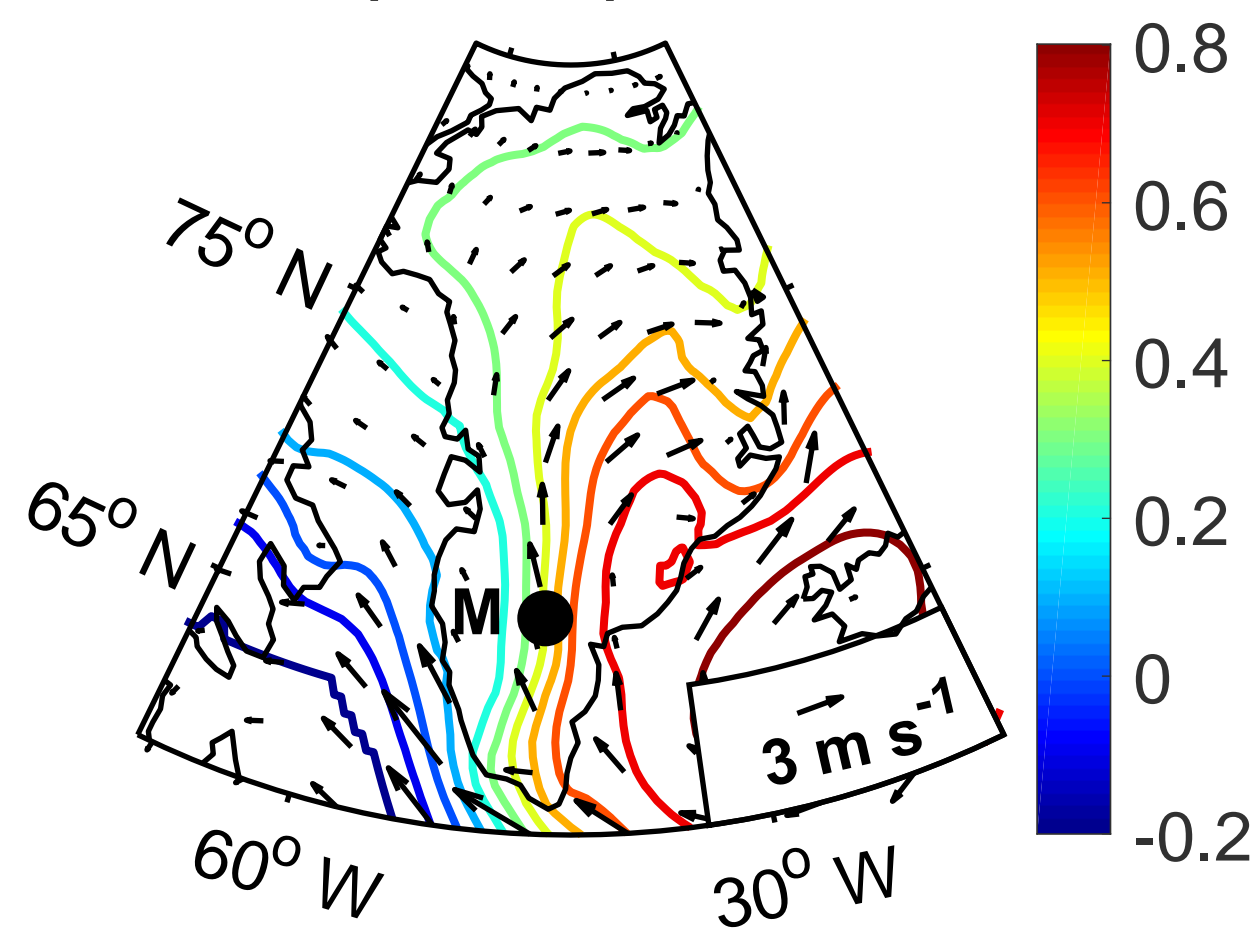
(c) SLP (norm.) and wind an.
