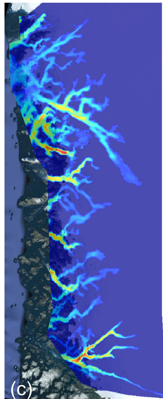
Mean frontal melt rate
