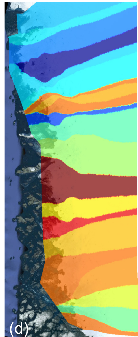
Calving threshold \sigma_{\max}
