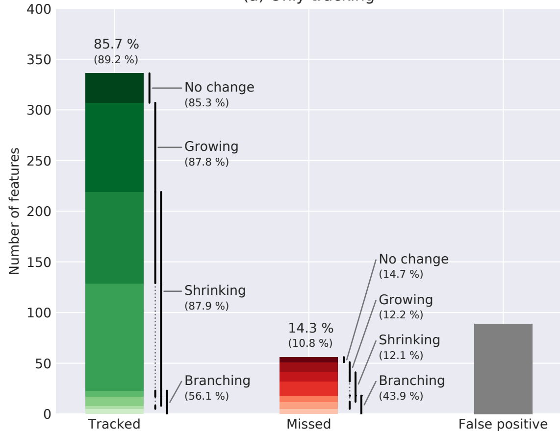
(a) Only tracking
