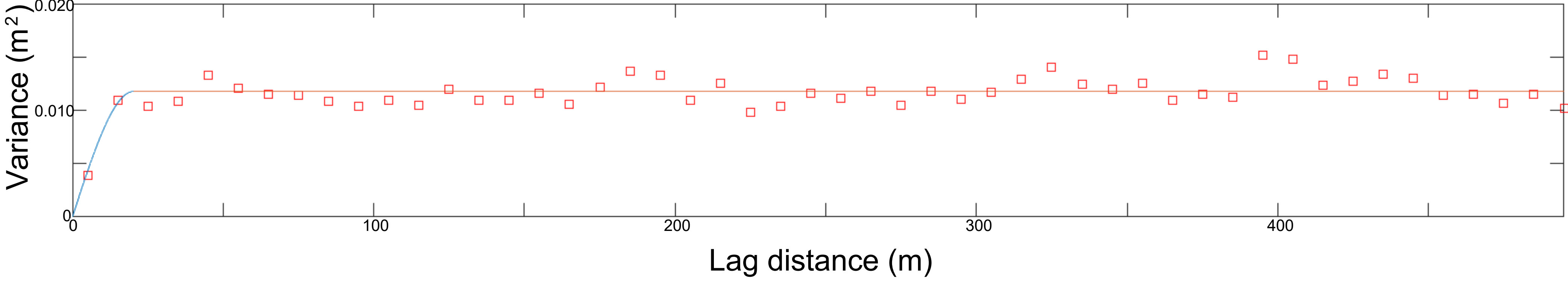
(c) Elevation differences between GPS A and ATM (10/26/2014)
