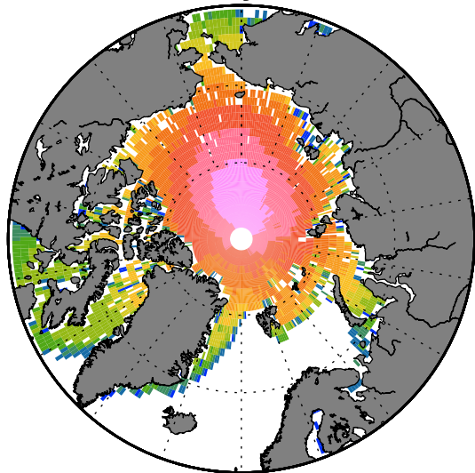
(a) CryoSat
