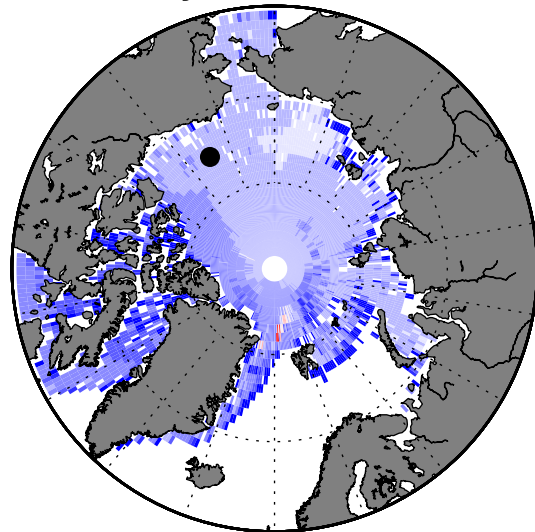
(c) CryoSat-PIOMAS
