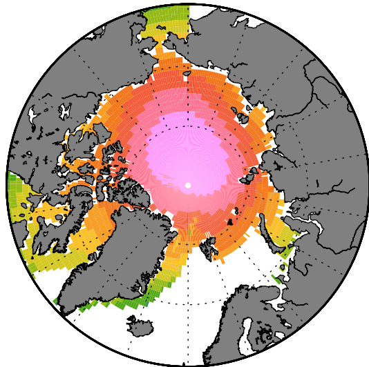
(b) PIOMAS
