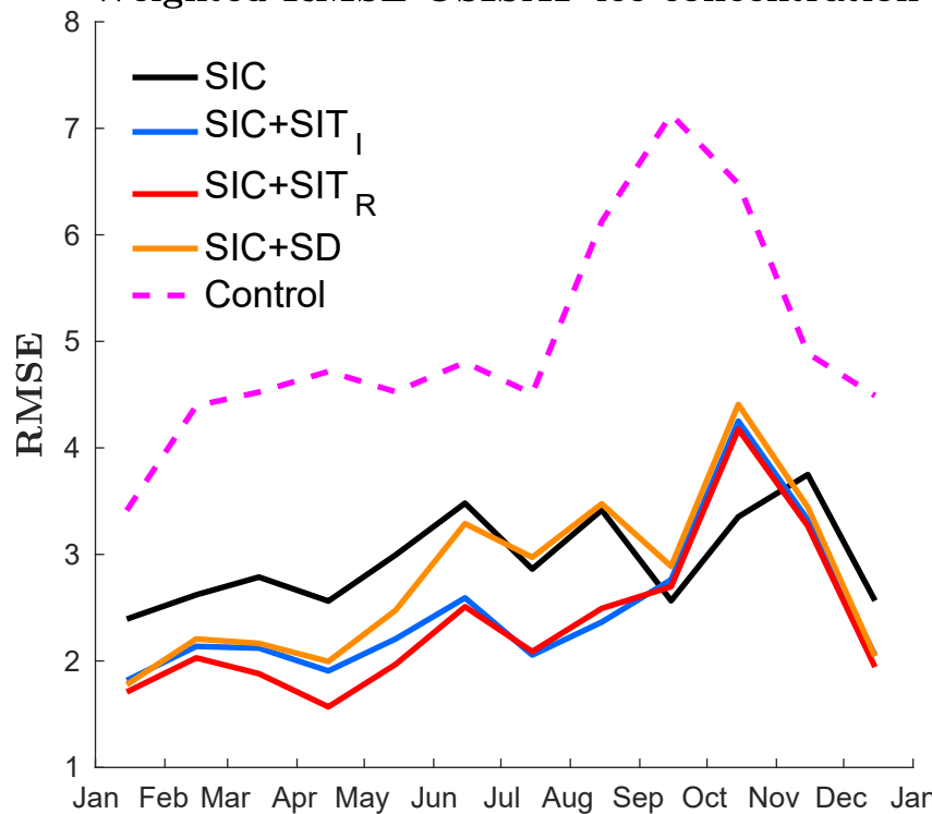
Weighted RMSE OSISAF ice concentration
