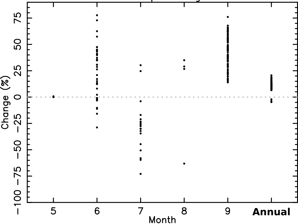
Change in fraction of subsurface runoff North Slope basin grids
