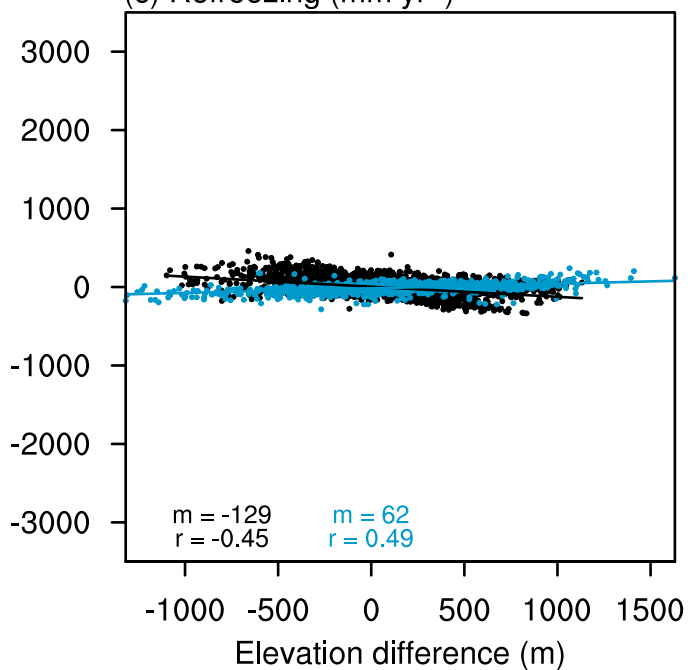
(c) Refreezing ( \text{mm yr}^{-1} )
