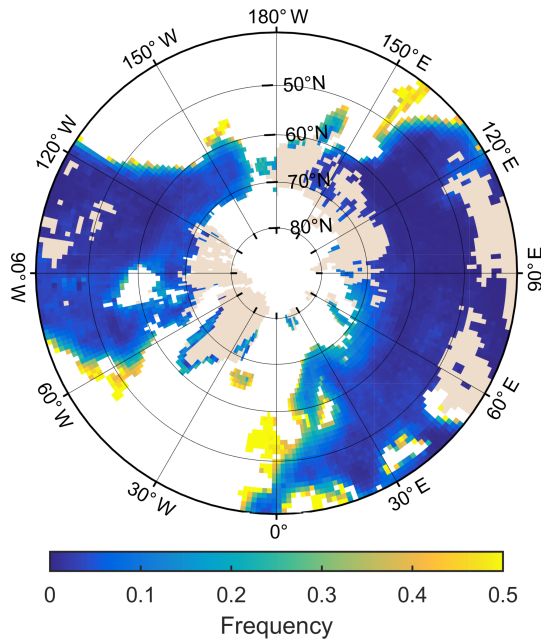
Figure 6. Frequency of days for 2004–2007 during which implementation of correction factors results in higher nighttime than daytime sub-canopy longwave radiation despite higher daytime than nighttime atmospheric longwave radiation.
