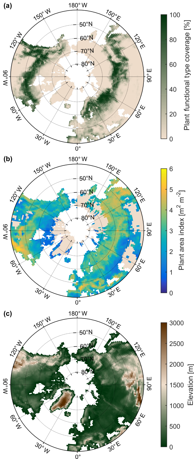
Figure 1. Coverage of vegetated land unit within grid cell by combination of needleleaf evergreen boreal trees (NEBTs) and needleleaf evergreen temperate trees (NETTs) (a), plant area index (PAI) for combination of NEBTs and NETTs weighted by PFT fractions (b), and grid-cell average elevation (c) based on CLM4.5’s 0.9^\circ \times 1.25^\circ surface dataset.
