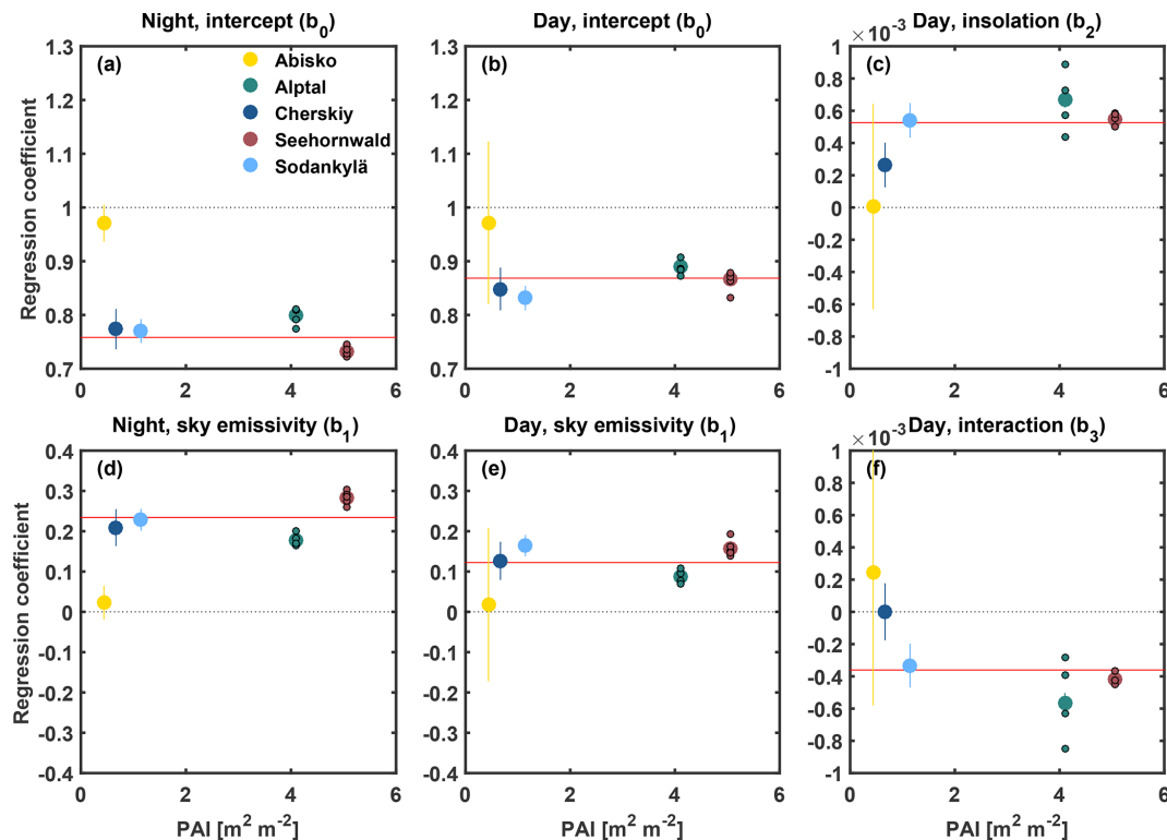
Figure 3. Regression coefficients (Eq. 6) for forest stands at Abisko (yellow), Alptal (green), Cherskiy (dark blue), Seehornwald (maroon), and Sodankylä (light blue), with small circles indicating individual seasons for Alptal and Seehornwald and solid lines indicating 95 % confidence intervals. Red lines display regression coefficients calculated from a combination of Alptal (season 2005), Cherskiy, Seehornwald (season 2009), and Sodankylä. Intercept b_0 and regression coefficient for \varepsilon_{\text{sky}} b_1 are differentiated for night (a and d, respectively) and day (b and e, respectively). Regression coefficient for insolation b_2 and regression coefficient for interaction of \varepsilon_{\text{sky}} and insolation b_3 are shown for day only (c and f, respectively). Regression coefficients involving insolation have the unit of square metres per watt ( \text{W}^{-1} \text{m}^2 ).
