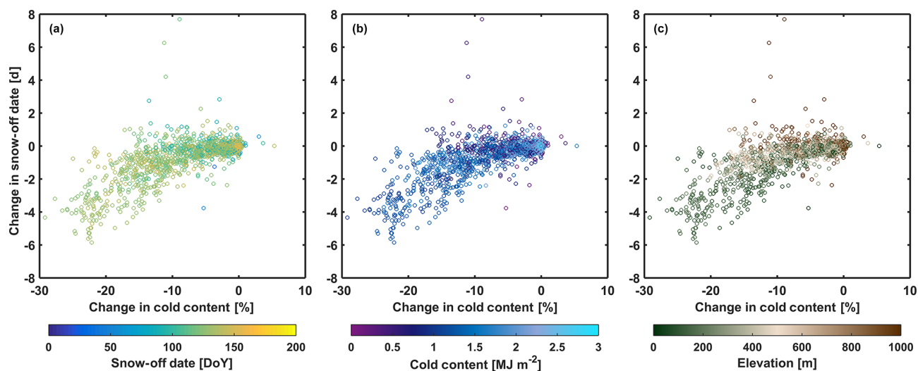
Figure 9. Change in cold content and snow-off date from CTRL to CORR as a function of (a) snow-off date and (b) cold content in CTRL as well as elevation (c) for grid cells within the area 42 to 70° N and 40 to 140° E.
