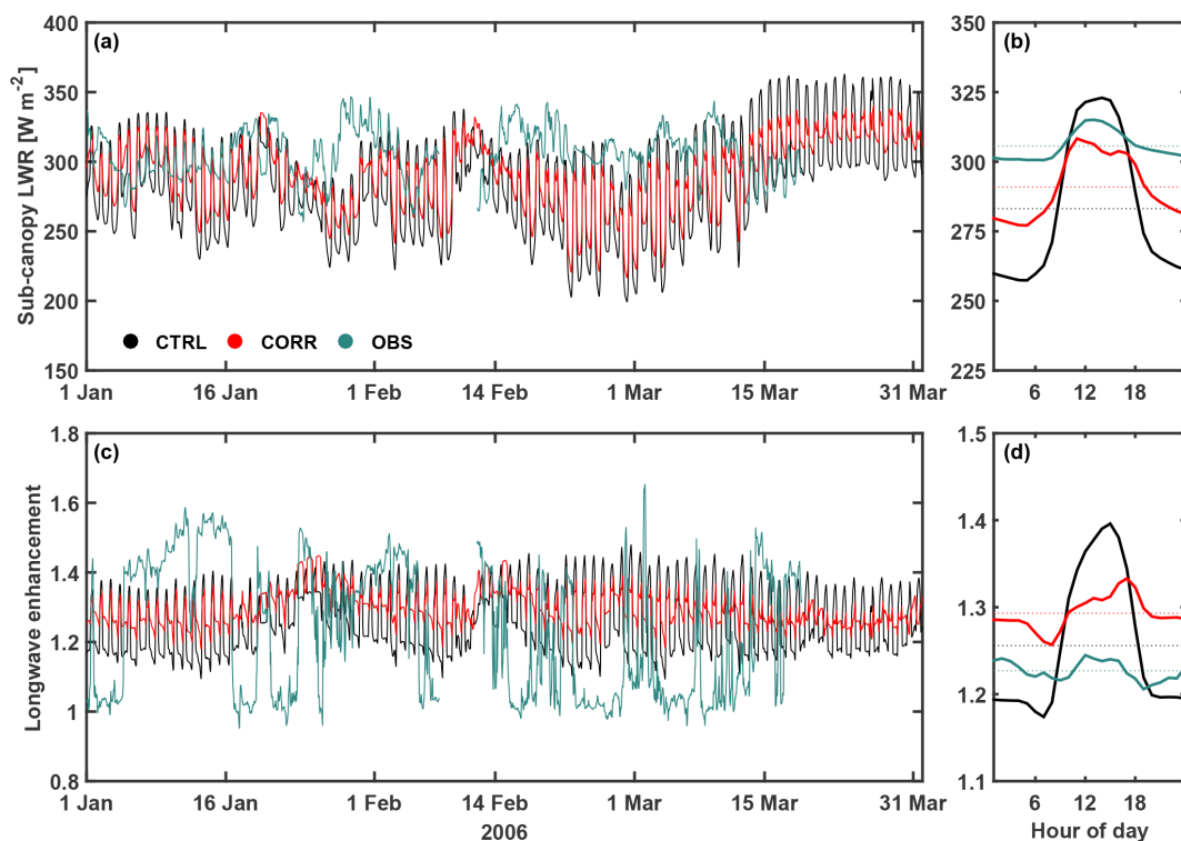
Figure 4. Hourly time series (a, c), diurnal cycles (solid in b and d), and JFM averages (dotted in b and d) of sub-canopy longwave radiation (a, b) and longwave enhancement (c, d) for the snowmelt season in 2006 at Alptal, Switzerland. Measurements at the forest stand (OBS; green) are shown for comparison with offline simulations CTRL (black) and CORR (red) for boreal evergreen needleleaf trees in the corresponding grid cell of Alptal, Switzerland. Gaps in measurements are due to quality checks and excluded from calculation of diurnal cycle and JFM average.
