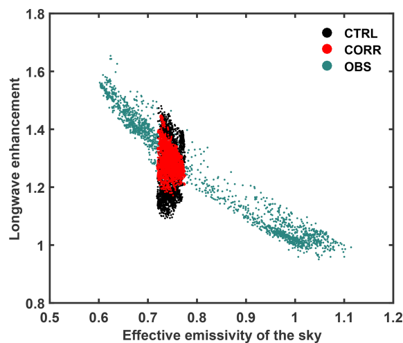
Figure 5. Longwave enhancement measured (OBS; green) at the forest stand of Alptal, Switzerland, and simulated in CTRL (black) and CORR (red) for boreal evergreen needleleaf trees in the corresponding grid cell of Alptal, Switzerland, as a function of effective emissivity of the sky. Each data point represents an hourly average seen in Fig. 4c.
