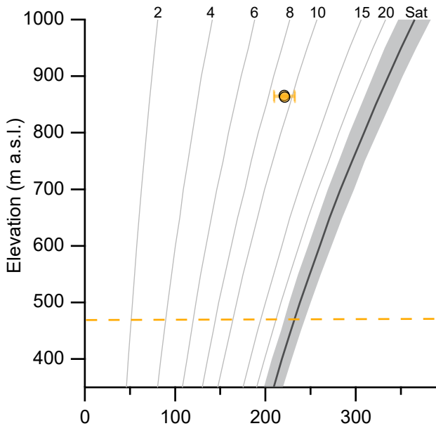
(a) C-14 concentration ( 10^3 atoms g^{-1} )
