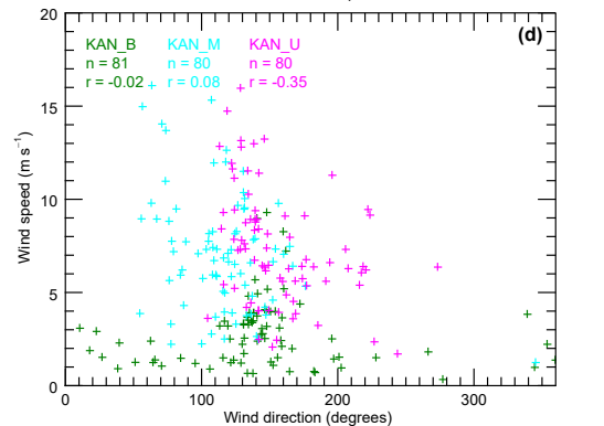
K-transect wind comparisons
