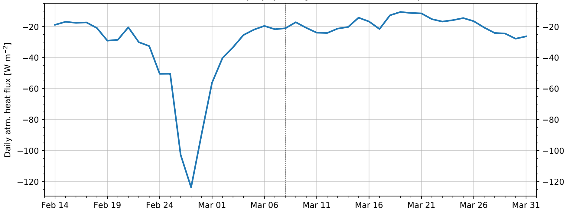
(b) NAOSIM heat flux in polynya (negative: ocean \rightarrow atmosphere)
