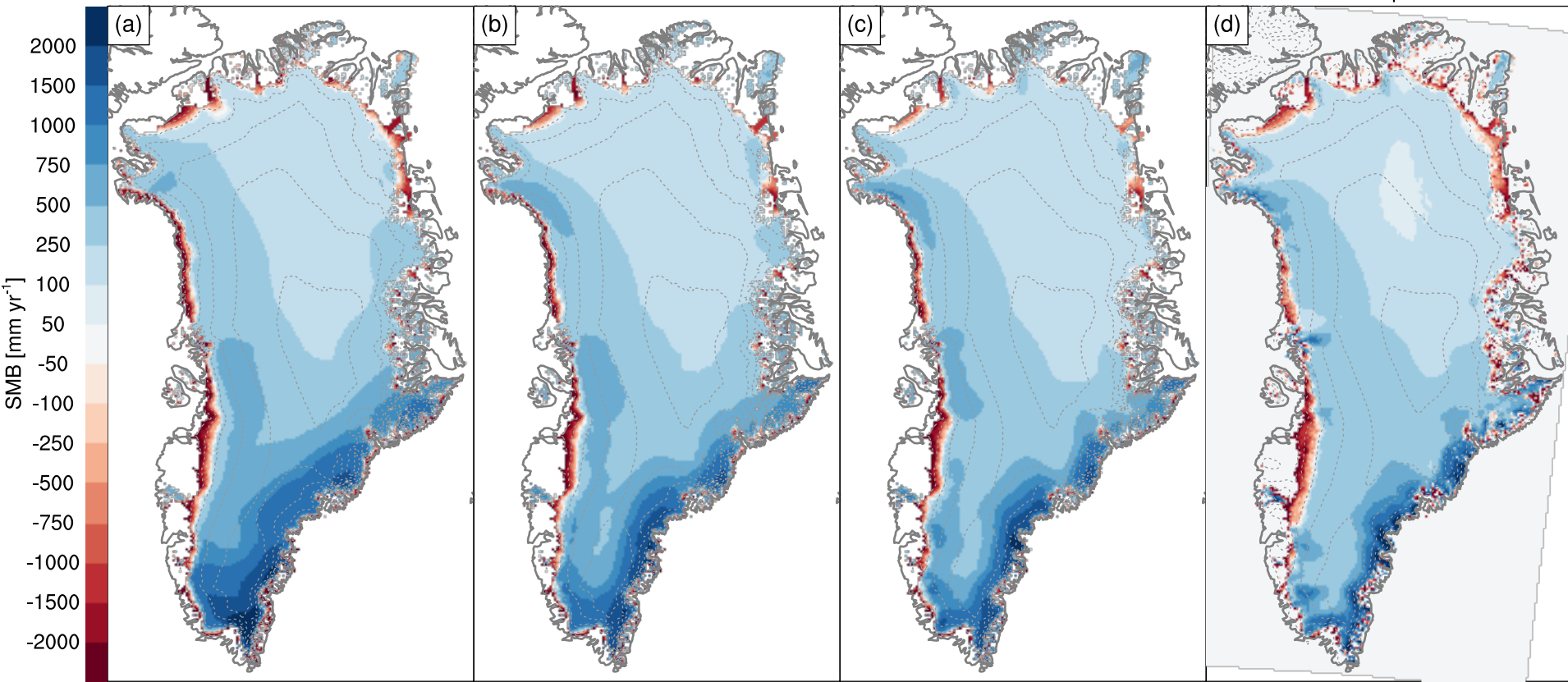
RACMO2.3p2 at 1 km
