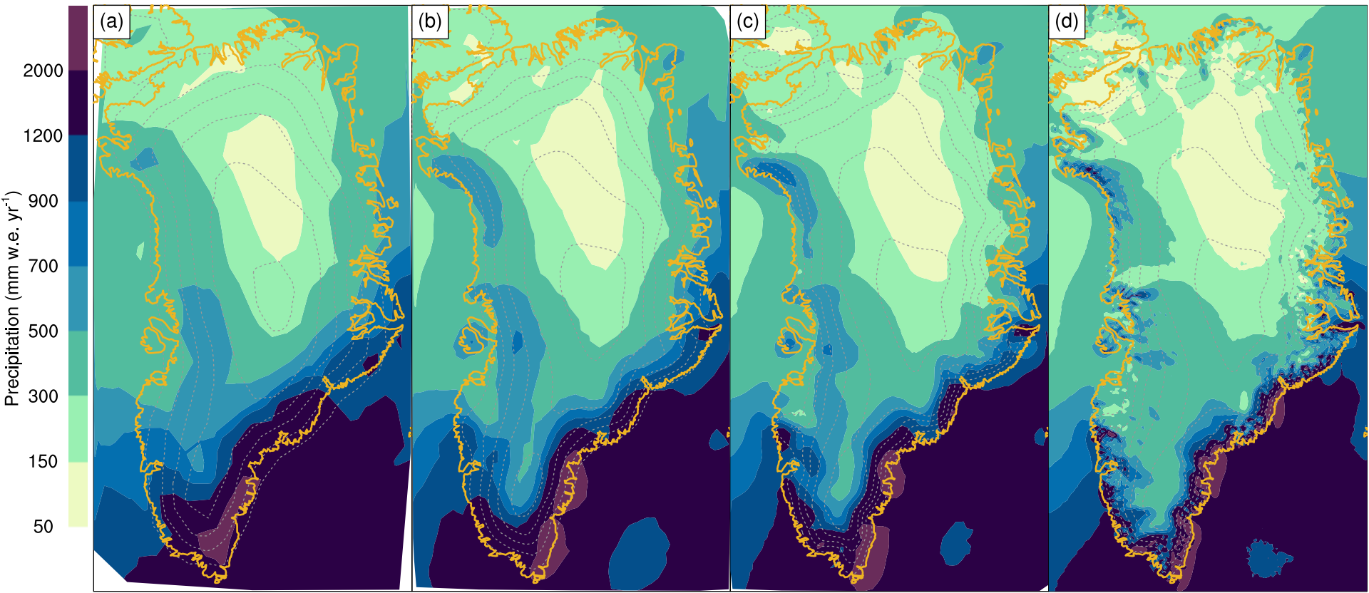
Uniform CESM 111 km
