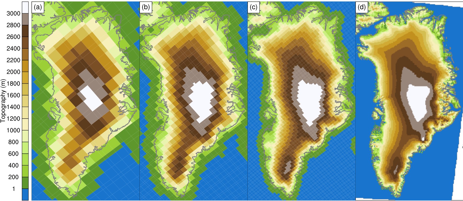
CESM uniform 111 km
