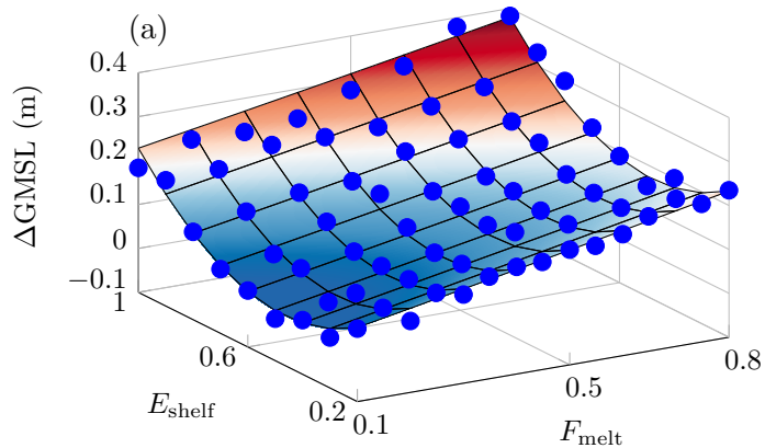
RCP 2.6 (2300)
