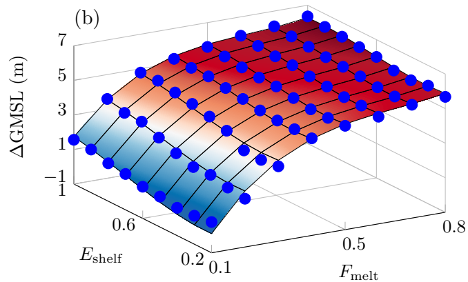
RCP 8.5 (3000)
