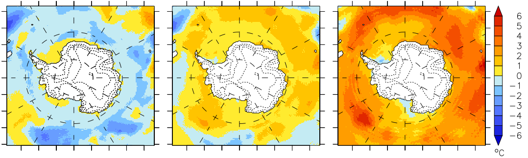
(a) SST(NorESM1-ME)
