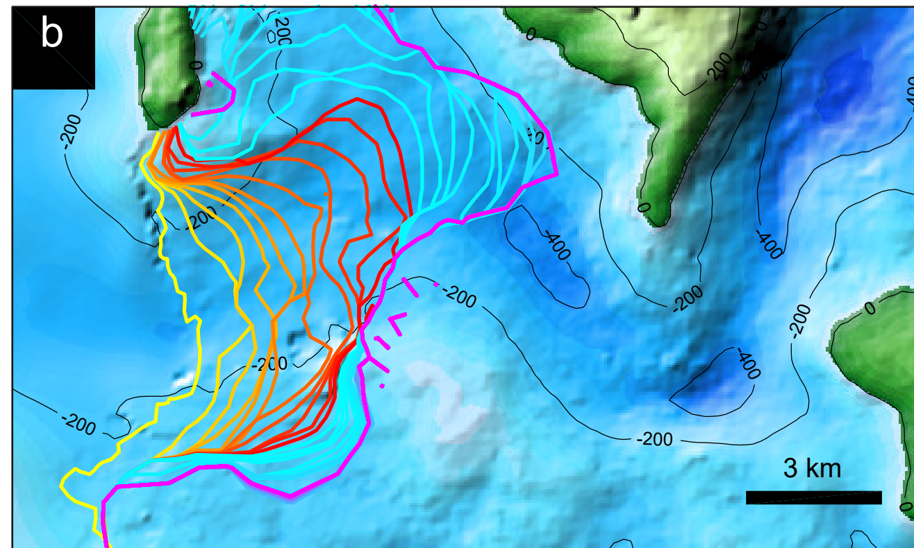
Height-above-buoyancy (HAB)
