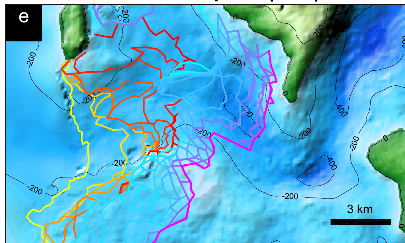
Crevasse-depth 2 (CD2)
