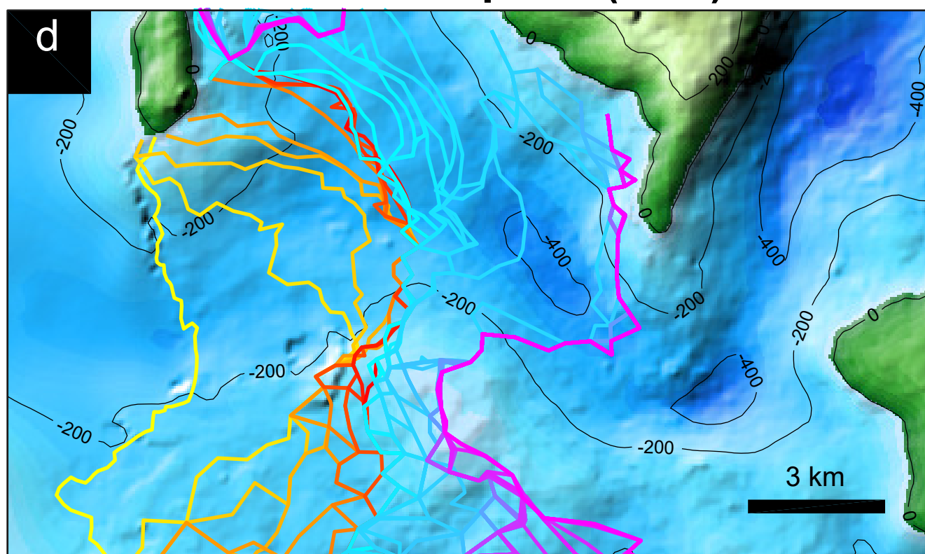
Crevasse-depth 1 (CD1)
