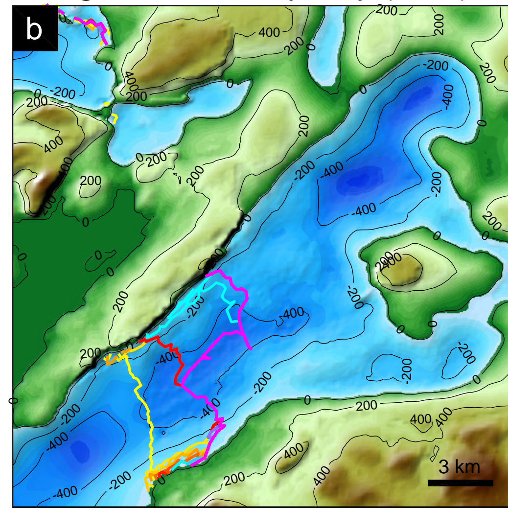
Height-above-buoyancy (HAB)
