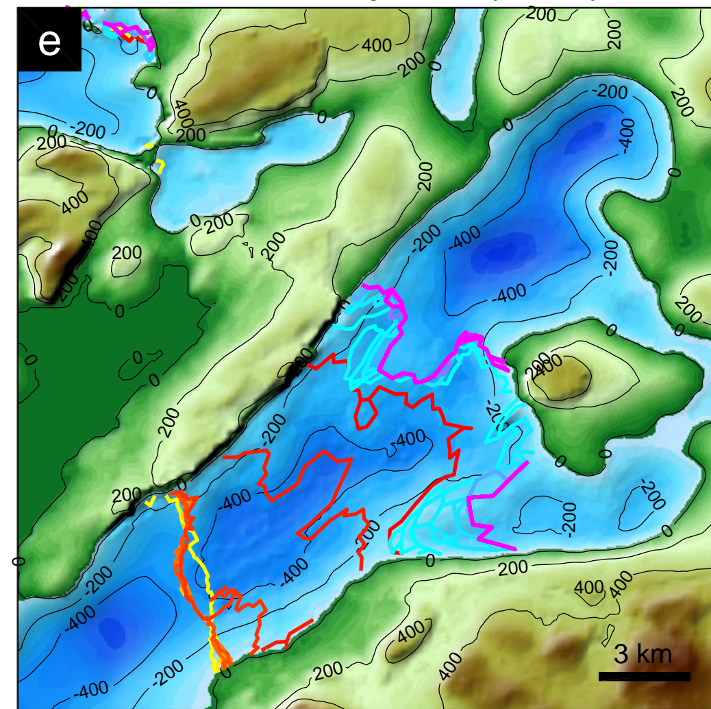
Crevasse-depth 2 (CD2)
