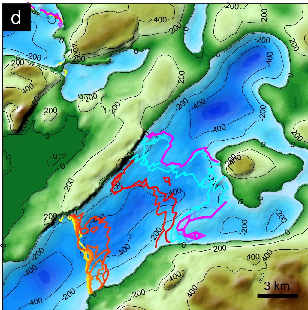
Crevasse-depth 1 (CD1)
