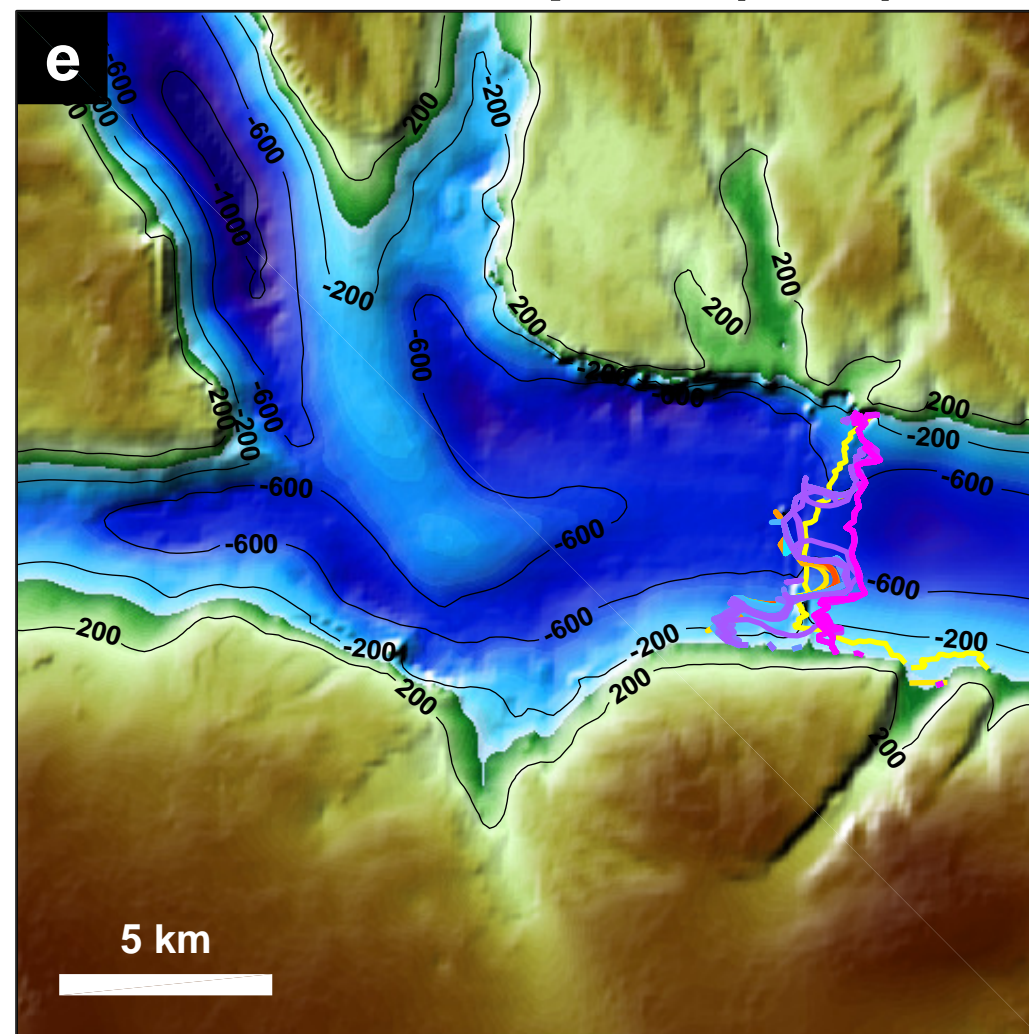
Crevasse-depth 2 (CD2)
