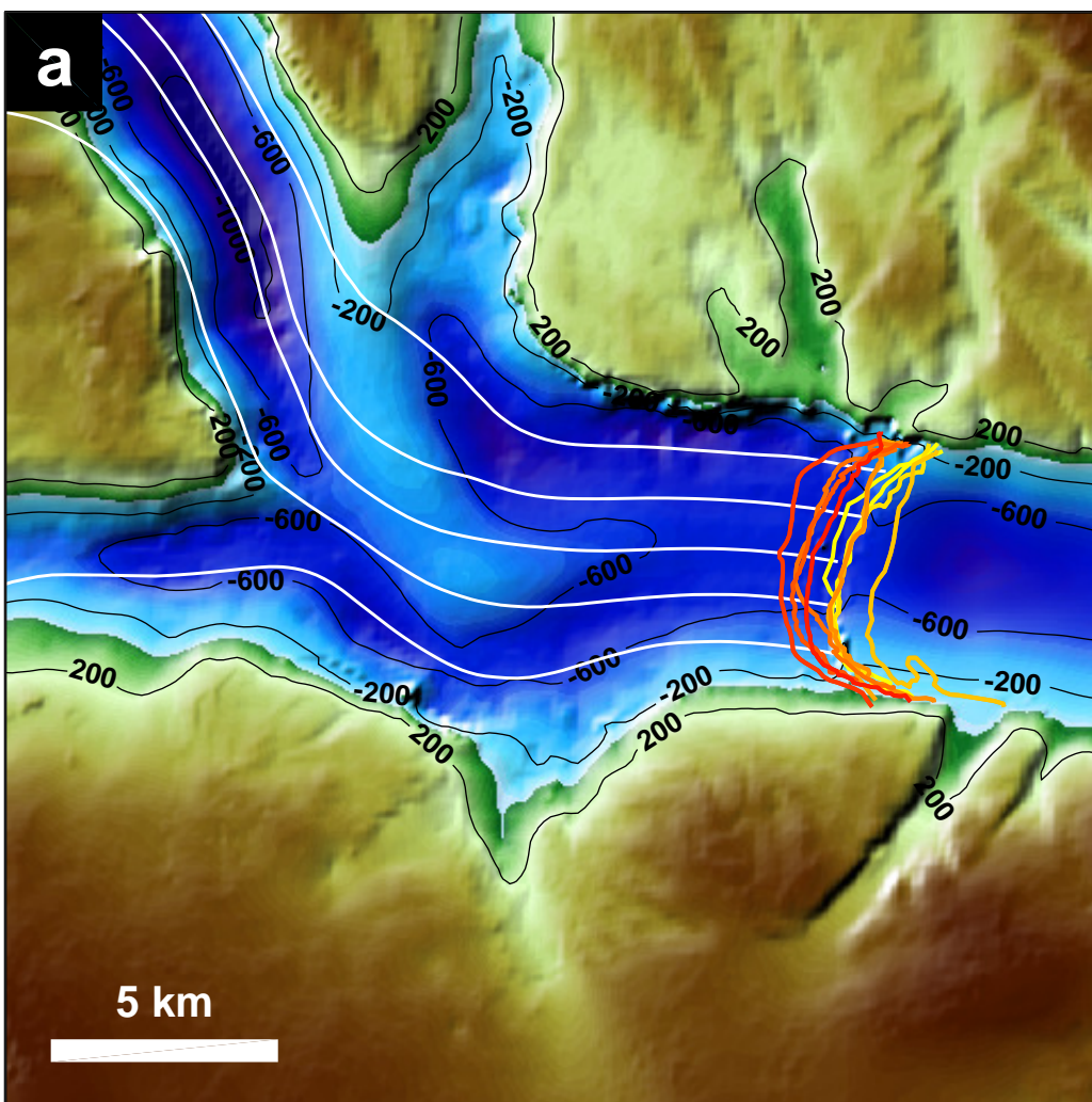
Observed ice front
