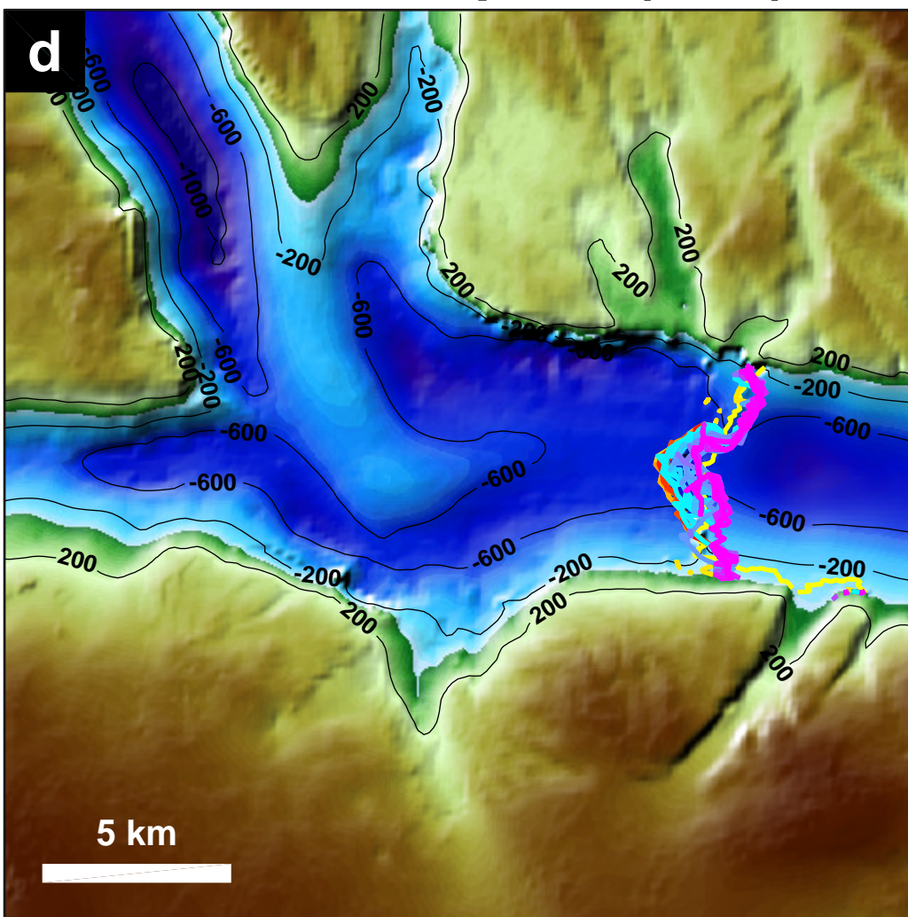
Crevasse-depth 1 (CD1)
