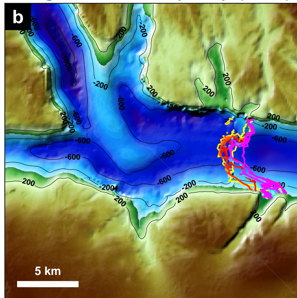
Height-above-buoyancy (HAB)
