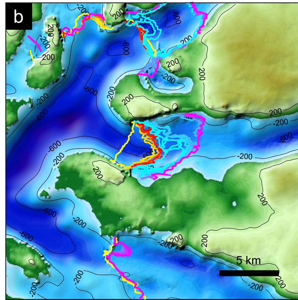
Height-above-buoyancy (HAB)
