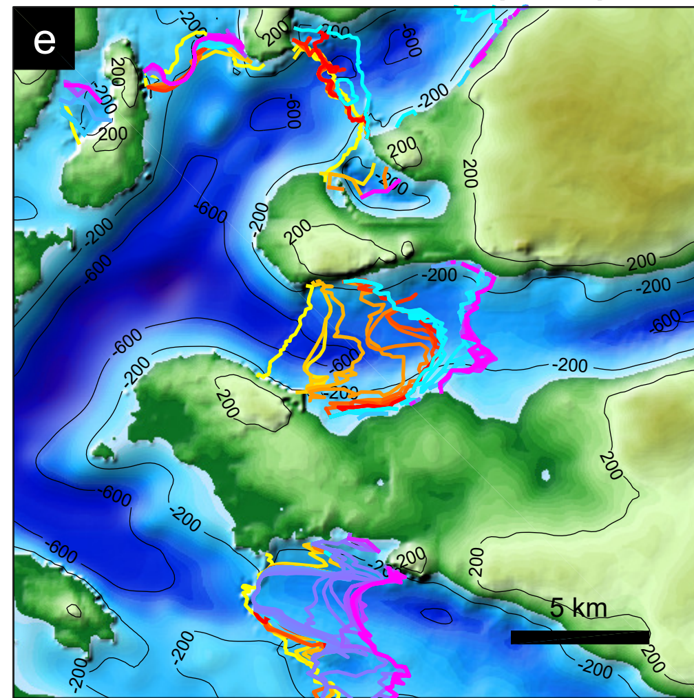
Crevasse-depth 2 (CD2)
