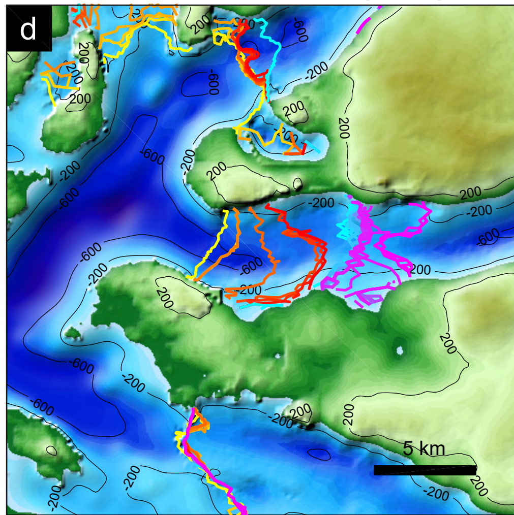
Crevasse-depth 1 (CD1)
