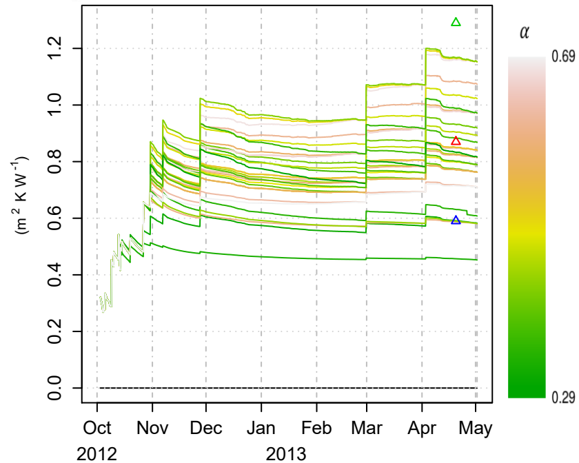
Bulk R_{th} at transect points
