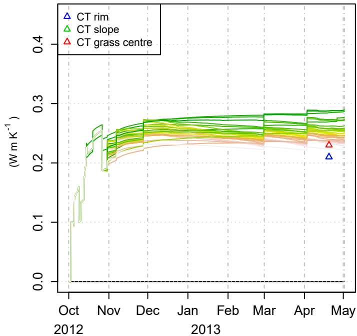
Bulk K_{eff-z} at transect points
