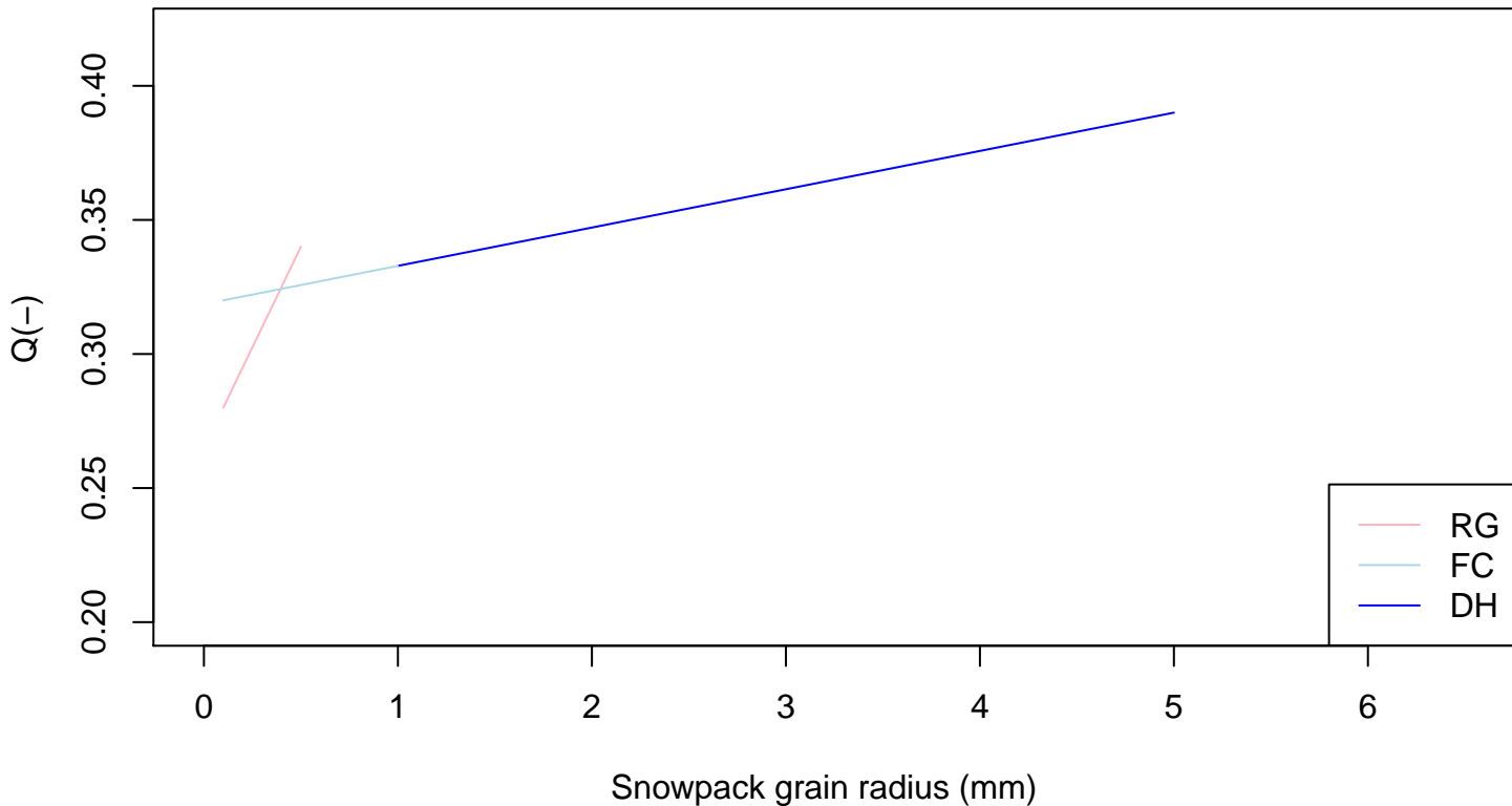
Q as a function of SNOWPACK grain size
