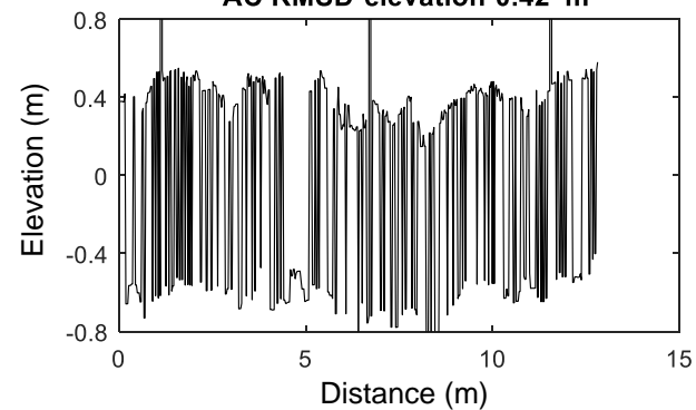
AC RMSD elevation 0.42 m
