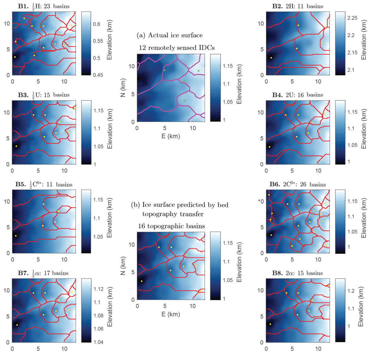
Figure 11. (a) IDCs (magenta outlines) and moulins (green dots) obtained from satellite images by Yang and Smith (2016). (b, B1–B8) Ice surface topographic basins (red outlines) and local minima (yellow dots) on ice surfaces predicted with bed topography transfer with various ice flow parameters. Study region R1 (Fig. 1a, Table 1) with \eta = 10^{14} Pa s and baseline C^{0*} = 10 . While the bed-transfer-predicted topographic basin configuration in (b) is different from the IDC configuration in (a), the basin densities are similar. Changing ice thickness H or basal sliding parameter C^{0*} by a factor of 2 produces significant changes in predicted topographic basin configurations (B1, B2 and B5, B6).
