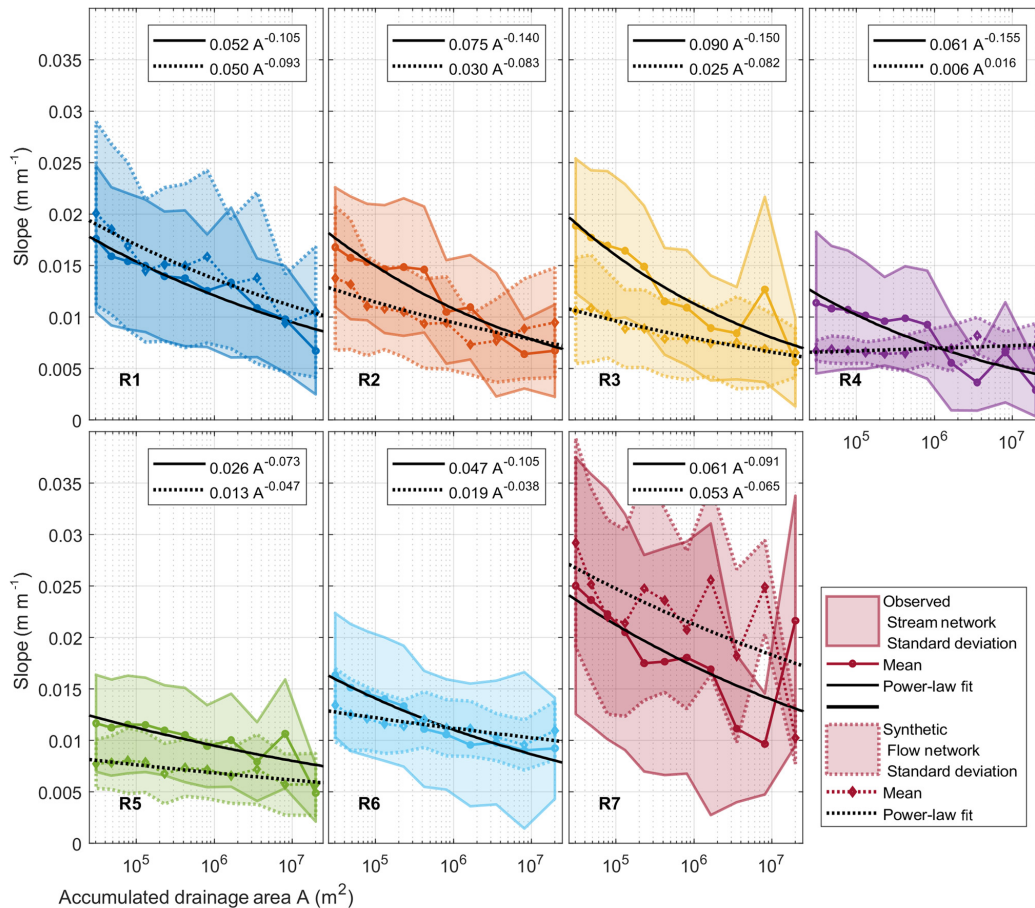
Figure 9. Mean stream channel slopes binned by accumulated upstream drainage–flow area from our seven study regions (Fig. 1a, Table 1). Results are shown from both observed supraglacial stream networks and synthetic flow networks calculated on surfaces predicted with bed topography transfer (see Sect. 2.4.2 and 2.4.3). The standard deviation of slope within each area bin is indicated by shaded patches, where patches with solid outlines correspond to observed stream networks and patches with dotted outlines to synthetic flow networks. Mean slopes are shown by solid and dotted colored lines and power-law fits by solid and dotted black lines. Under the (likely inaccurate) assumptions that supraglacial stream longitudinal elevation profiles are incisionally controlled and in a steady-state configuration under ice flow conditions analogous to uniform uplift, the power-law fit coefficients and exponents should correspond to K^{-1} and -m from Eq. (7). Synthetic flow networks from regions R3 to R5 and R6 may not be meaningful due to surface underprediction (see Sect. 3.2).
