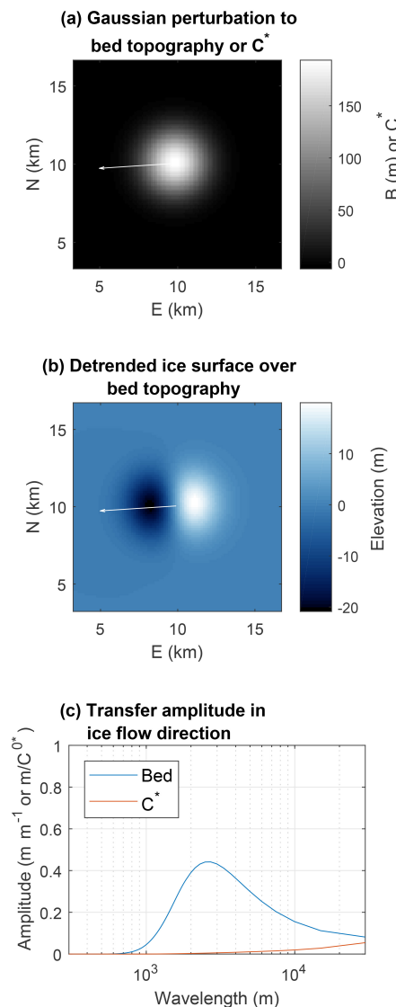
Figure 4. Illustration of steady-state basal transfer for ice flow parameters representative of the western Greenland ablation zone. Ice flow parameters are from region R1 (Fig. 1a, Table 1) with \eta = 10^{14} \text{ Pa s} . (a) Gaussian bed topography or basal sliding perturbation. (b) Detrended predicted ice surface over the Gaussian bed topography perturbation (with C^{0*} = 10 ). White arrows in (a) and (b) indicate the ice flow direction. (c) Transfer amplitudes in the ice flow direction (along a flow line) for bed topography and basal sliding C^{0*} perturbations. The transfer functions also have important phase components not shown here (see Gudmundsson, 2003). With these flow parameters, surface topography created from basal sliding perturbations should generally be of much lower amplitude than surface topography created from bed topography.
