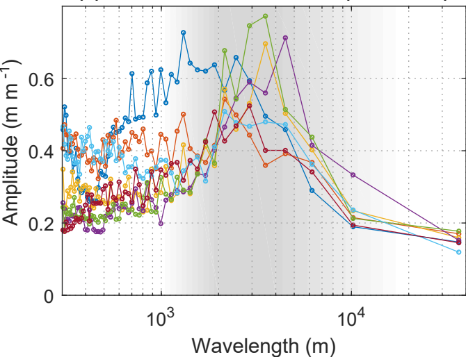
(c) Surface/bed admittance (flow lines)
