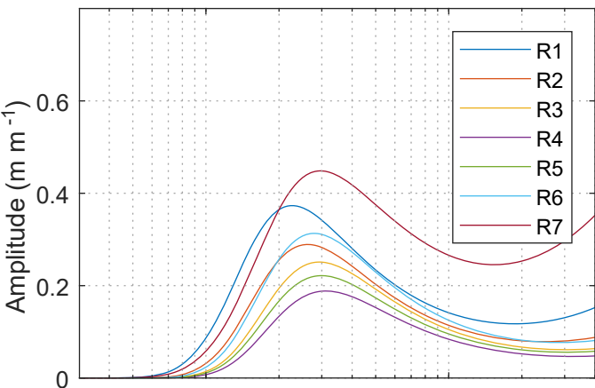
(b) Ice surface/bed admittance (2-D DFTs)
