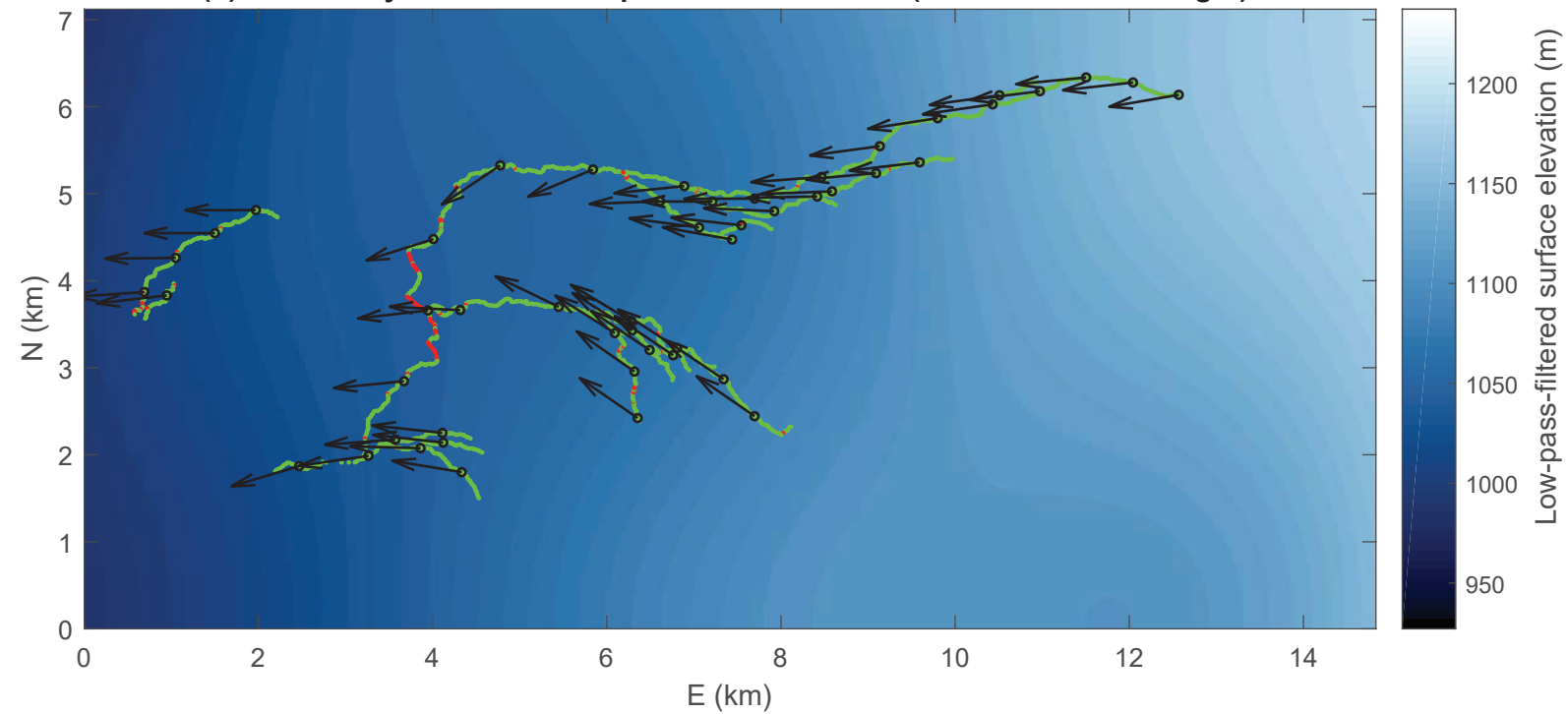
(b) Conformity metrics on low-pass-filtered surface (6 km cutoff wavelength)
