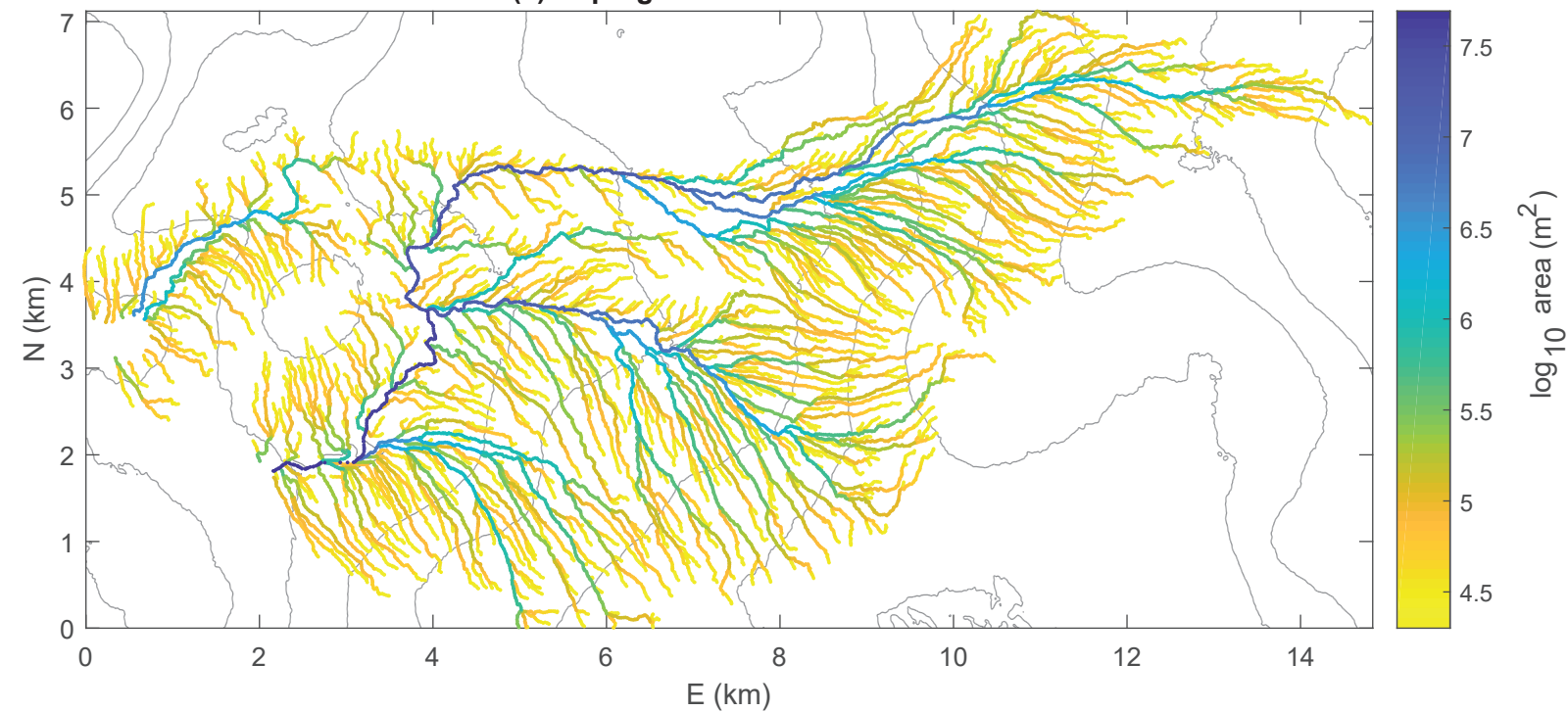
(a) Supraglacial stream network
