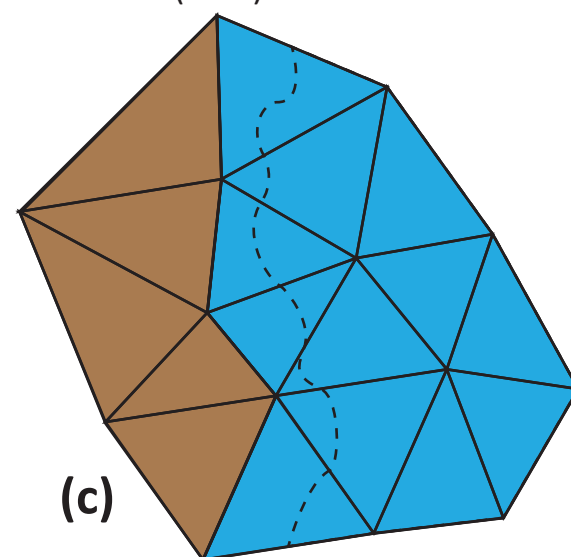
Full melt parameterization (FMP)
