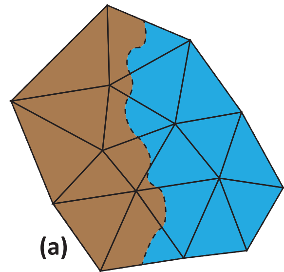
Exact grounding line position
