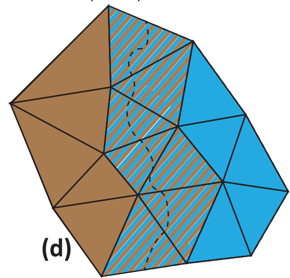
Sub-element melt 1 (SEM1)
