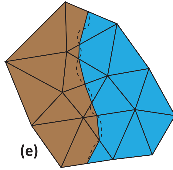
Sub-element melt 2 (SEM2)
