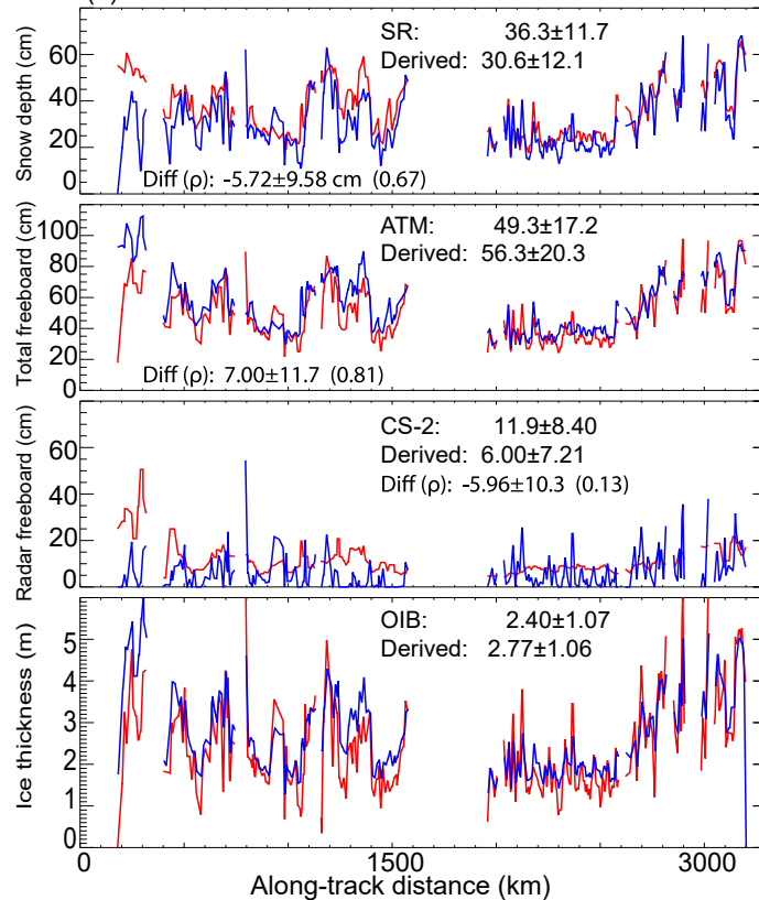
(a) 2011 Oct 11
