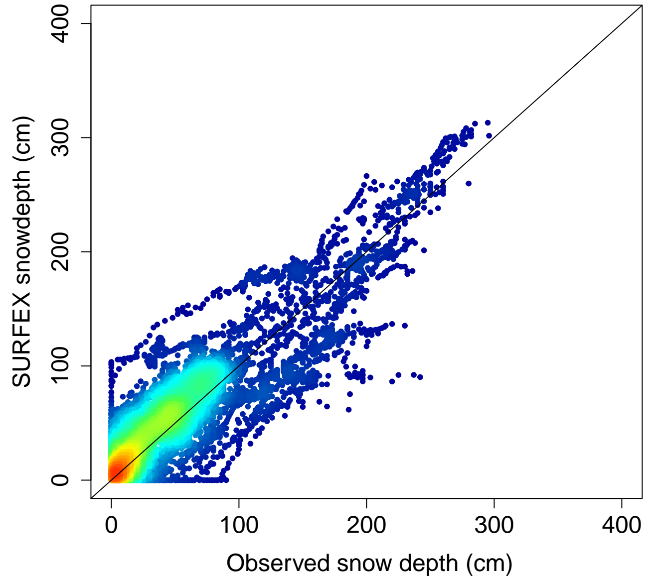
(b) GridObs–Crocus
