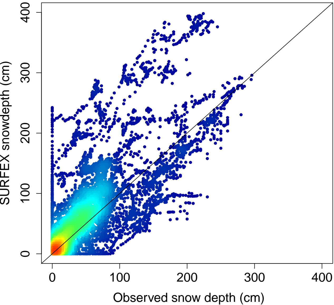
(a) AROME–Crocus
