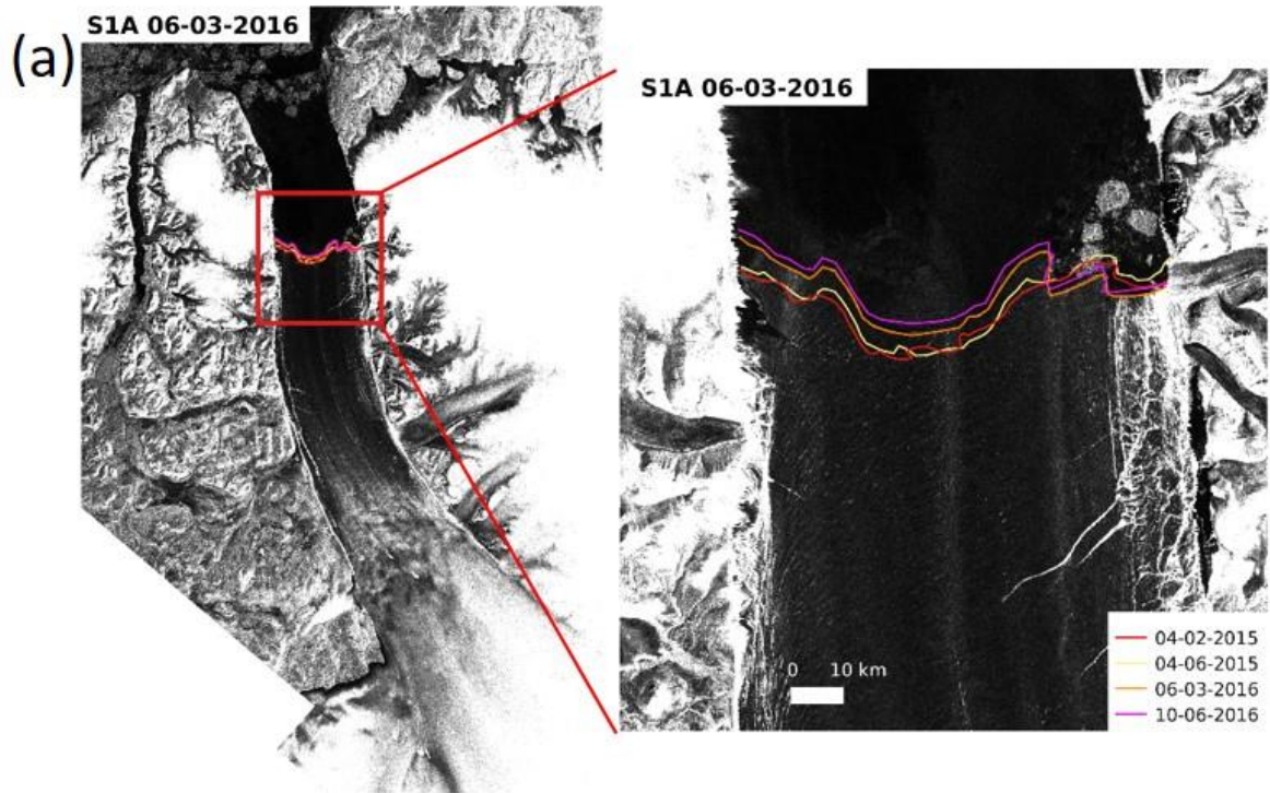
Figure S1: Ice front location extracted from Sentinel-1 images on (a) Petermann Glacier and (b) Nioghalvfjærdssjorden.
