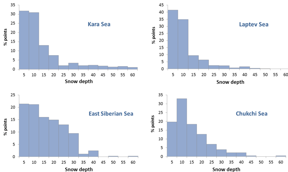
Figure 6. Distribution of snow depth on the level ice in the marginal seas.
