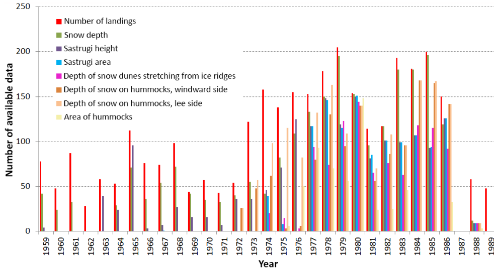
Figure 3. The number of landings and the number of different snow observations per year carried out in the MAM months.
