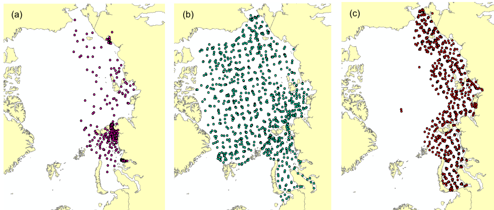
Figure 2. Sever expedition landings where snow measurements were conducted in the MAM months: 1960s (a), 1970s (b) and 1980s (c).
