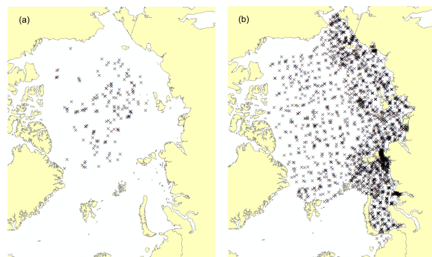
Figure 1. Monthly mean positions of NP drifting stations in 1954–1991 (a) and Sever expedition landings where snow measurements were conducted in 1959–1986 (b). Only observations in the MAM months are shown for both sets of measurements.
