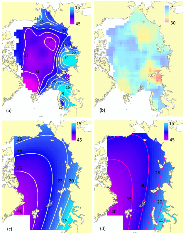
Figure 11. Map of snow cover depth (in cm) on the sea ice in the MAM months in 1959–1988: (a) gridded data with the grid cell 100x100 km and contour lines overlaid on it, (b) standard deviation of the data used for gridding, (c) map produced from the same data as (a), but using two-dimensional quadratic fit shown by Eq. (3), (d) Warren climatology averaged for the MAM months.
