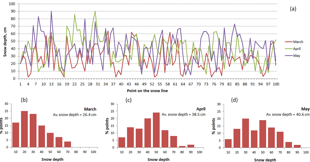
Figure 10. (a) Snow line measurements made in 1969 in the MAM months during the work of NP16 drifting station. The length of snow line was 1 km. (b–d) Distributions of measured snow depths in March, April and May 1969.
