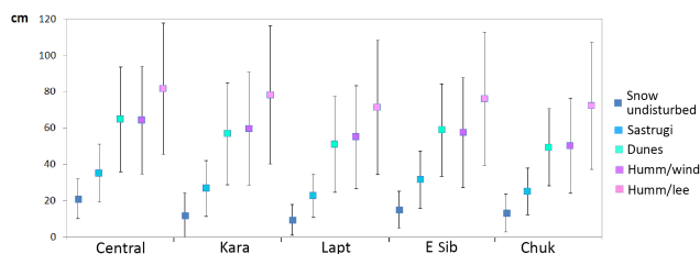
Figure 14. Sever snow depth observation statistics in the MAM months: depth of undisturbed snow on the level ice, snow depth of sastrugi, snow depth of dunes extending out from ice ridges, depth of snow on windward and leeward sides of the hummock and corresponding standard deviations. Data shown are averages for the central Arctic and for the four seas: Kara, Laptev, East Siberian and Chukchi.
