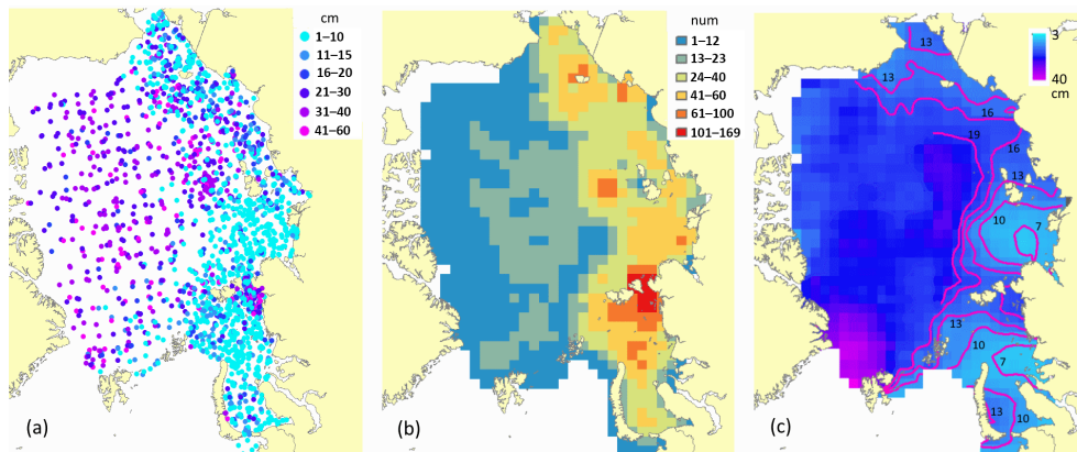
Figure 5. (a) Spatial distribution of measured snow depth on the level ice around Sever landing sites, MAM months, 1959–1988. (b) Number of point measurements used in gridding, grid cell is 100 \times 100 km. (c) Contour lines of the snow depth in the marginal seas produced using observations shown in panel (a). Snow depth is in cm.
