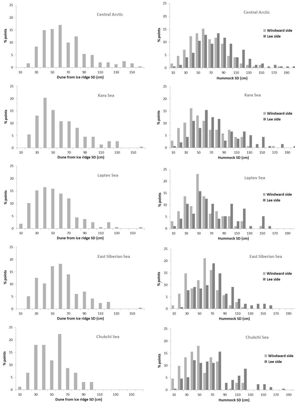
Figure 9. Distribution functions of snow depth (SD) in the dunes attached to ice ridges and around hummocks (on the windward and lee side) in different parts of the Arctic.
