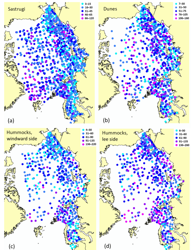
Figure 8. Height of sastrugi (a), depth of snow dunes extending out from ice ridges measured at a mid-length of a dune (b), snow depth on hummocks measured on the windward side (c) and snow depth on hummocks measured on the lee side (d), in cm. All observations were made in the MAM months.
