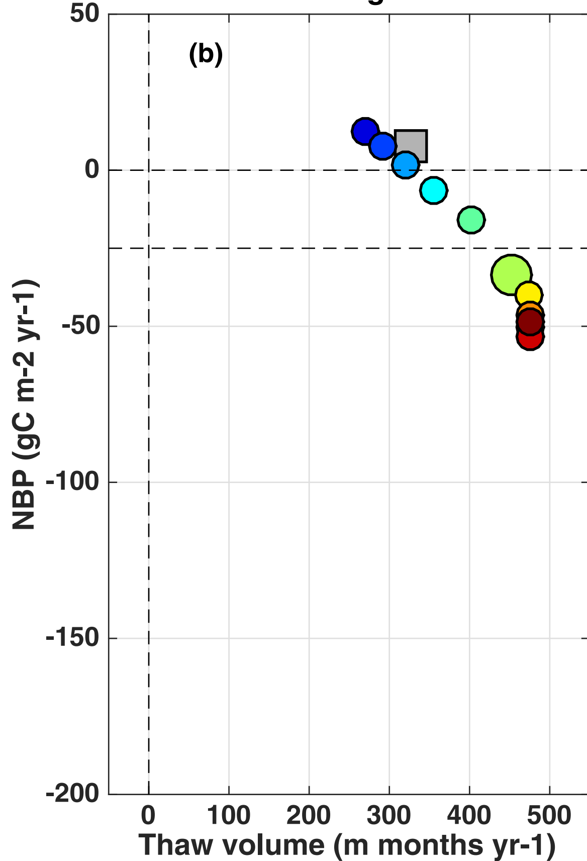
C source lags talik
