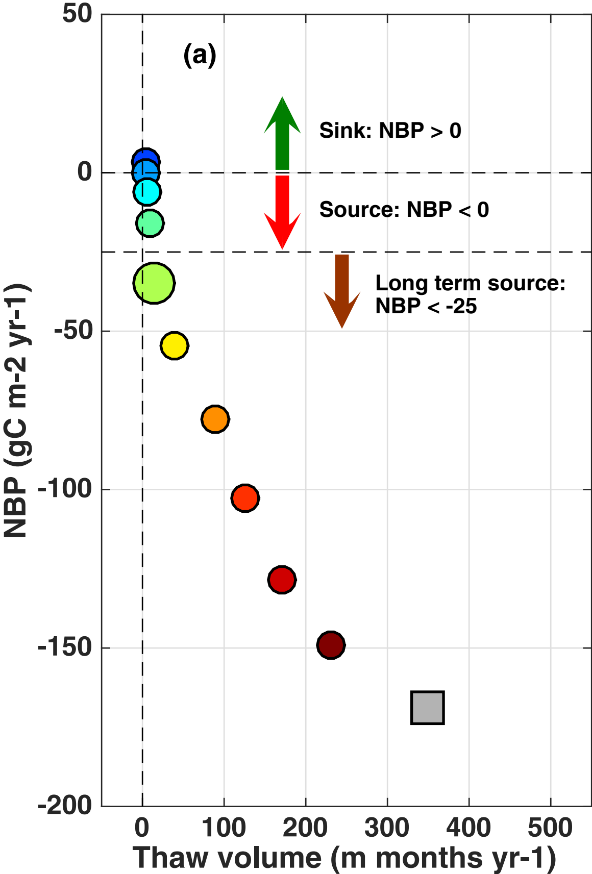
C source leads talik
