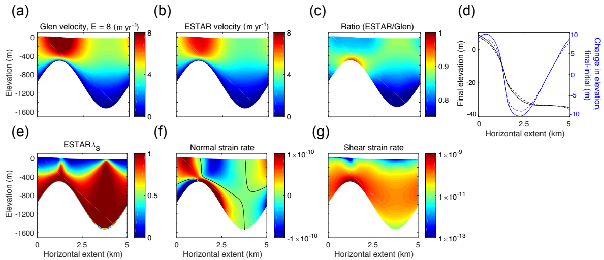
Figure 7. As for Fig. 6, but with L = 5 km.
