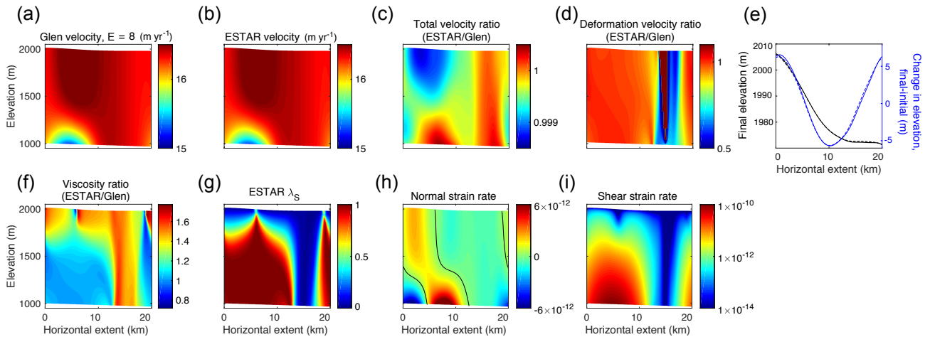
Figure 8. ISMIPDp full-Stokes steady-state results with horizontal extent L = 20 km. (a) Glen horizontal velocity v_x ( \text{m yr}^{-1} , with E_G = 8 ); (b) ESTAR v_x ( \text{m yr}^{-1} ); (c) ratio of ESTAR/Glen v_x ; (d) ratio of ESTAR/Glen deformation v_x ; (e) steady-state surface elevation (black) and difference between steady state and initial surface elevation (blue) for ESTAR (solid) and Glen (dashed); (f) ratio of ESTAR/Glen viscosity; (g) ESTAR \lambda_S ; (h) ESTAR normal strain rate ( \text{s}^{-1} ); and (i) ESTAR shear strain rate ( \text{s}^{-1} ). The black contours in (h) correspond to the curves where \dot{\epsilon}_{xx} = 0 . Note the log scale in (i).
