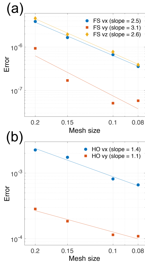
Figure 2. Convergence rates of the simulated (a) full-Stokes (FS) and (b) higher-order (HO) velocity fields ( v_x , v_y , v_z ) to the analytical solutions in Eqs. (13)–(17) for increasing mesh resolutions.
