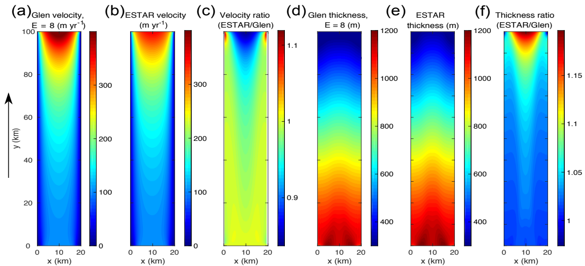
Figure 3. Rectangular ice shelf higher-order steady-state surface fields. (a) Velocity magnitude ( \text{m yr}^{-1} ) for the Glen flow relation ( E_G = 8 ); (b) velocity magnitude ( \text{m yr}^{-1} ) for ESTAR; (c) ratios (i.e. ESTAR/Glen) of velocity magnitudes; (d) thickness (m) for the Glen flow relation ( E_G = 8 ); (e) thickness (m) for ESTAR; and (f) ratios (i.e. ESTAR/Glen) thicknesses. The black arrow indicates the direction of flow.
