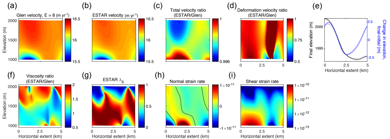
Figure 9. As for Fig. 8, but with L = 5 km.
