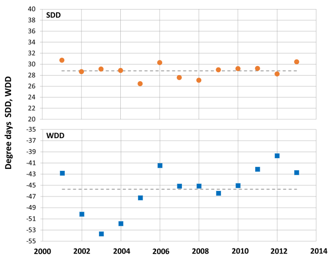
Figure 7. Summer degree days (SDD, circles) and winter degree days (WDD, squares) as an indicator for the thermal conditions at the ground surface over the course of the study period. The dashed lines indicate the respective means over the time period.
