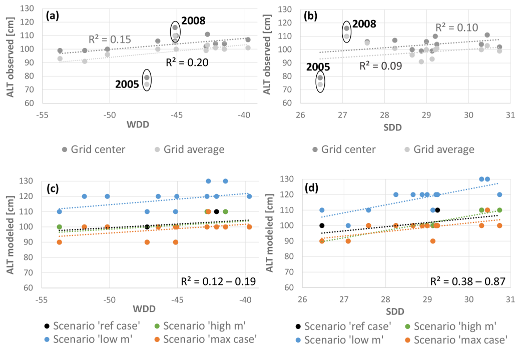
Figure 6. (a, b) Correlation of observed and (c, d) modelled active layer thicknesses to thermal conditions at the ground surface, considering winter degree days (WDD) and summer degree days (SDD) separately. Observed active layer measurements include information both from the grid centre (dark grey) and the grid average (light grey). Modelled active layer thickness is shown for selected scenarios “ref case” (black), “low m ” (blue), “high m ” (green), and “max case” only (orange).
