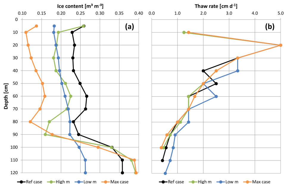
Figure 5. Comparison of (a) simulated ice content distribution with depth at the end of winter 2011 (1 May 2011) and (b) the corresponding modelled rate of active layer thaw starting after the first day of positive ground surface temperatures (25 May 2011), exemplified by four selected model scenarios.
