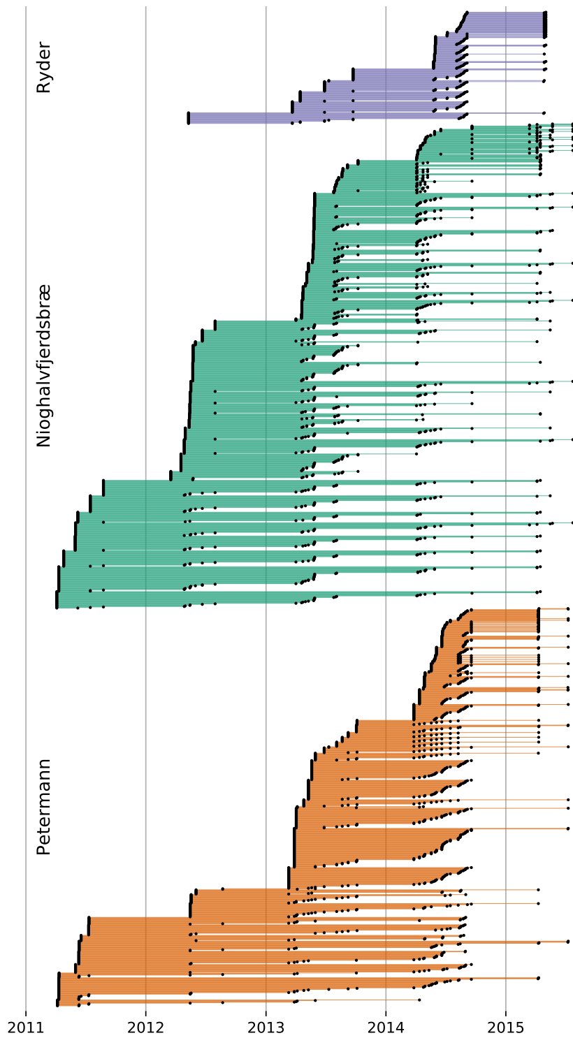
Figure 2: Timelines of DEM pairs for the three ice tongues considered, with each horizontal mark representing a difference computed between two DEMs.
