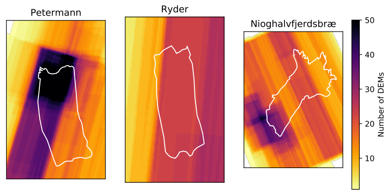
Figure 1: DEM coverage of the three ice tongues considered, with shading indicating the number of DEMs available, 2011–2015.
