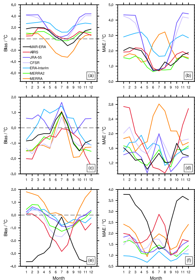
Figure 3. Mean over station-months of bias (a, c, e) and absolute error (b, d, f) relative to monthly mean SAT at: ice sheet stations above 1500 m (a, b); ice sheet stations below 1500 m (c, d); and coastal (DMI) stations (e, f). Ice sheet stations are from GC-Net, PROMICE and K-transect. All available station months from 1979 onwards are used. All datasets included in this figure are elevation corrected: several shorter reanalyses, AIRS, and MAR-ERA. Note that the vertical scales vary with panels.
