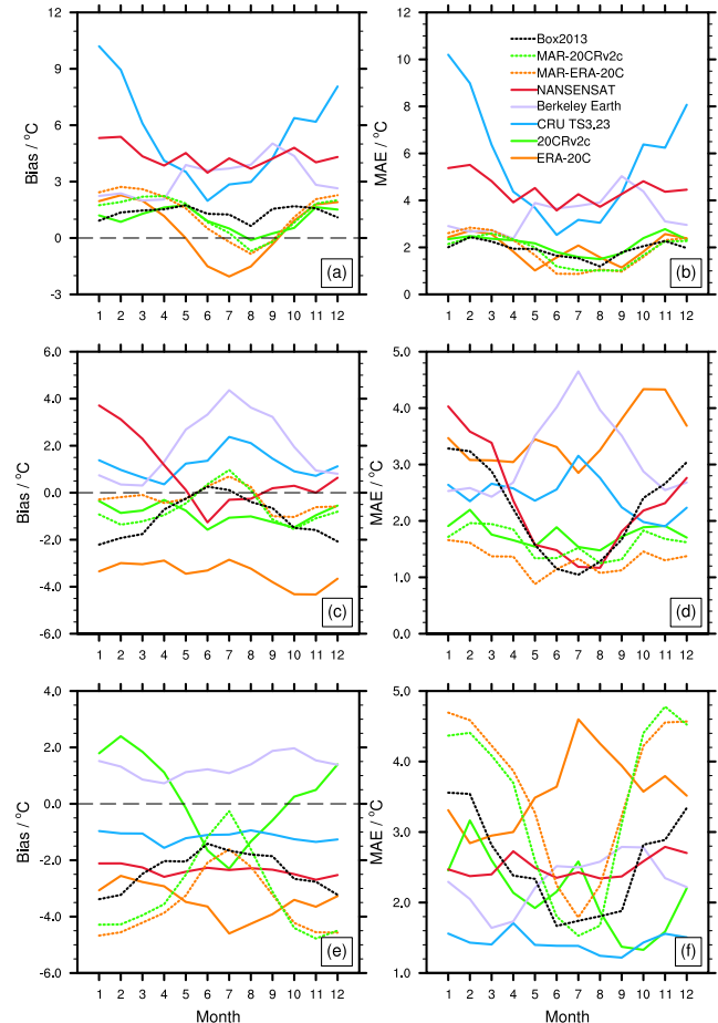
Figure 4. As in Fig. 3, but for elevation-corrected long reanalyses, MAR-ERA-20C and MAR-20CrV2C, Box2013 data and three gridded SAT analyses (not elevation corrected).
