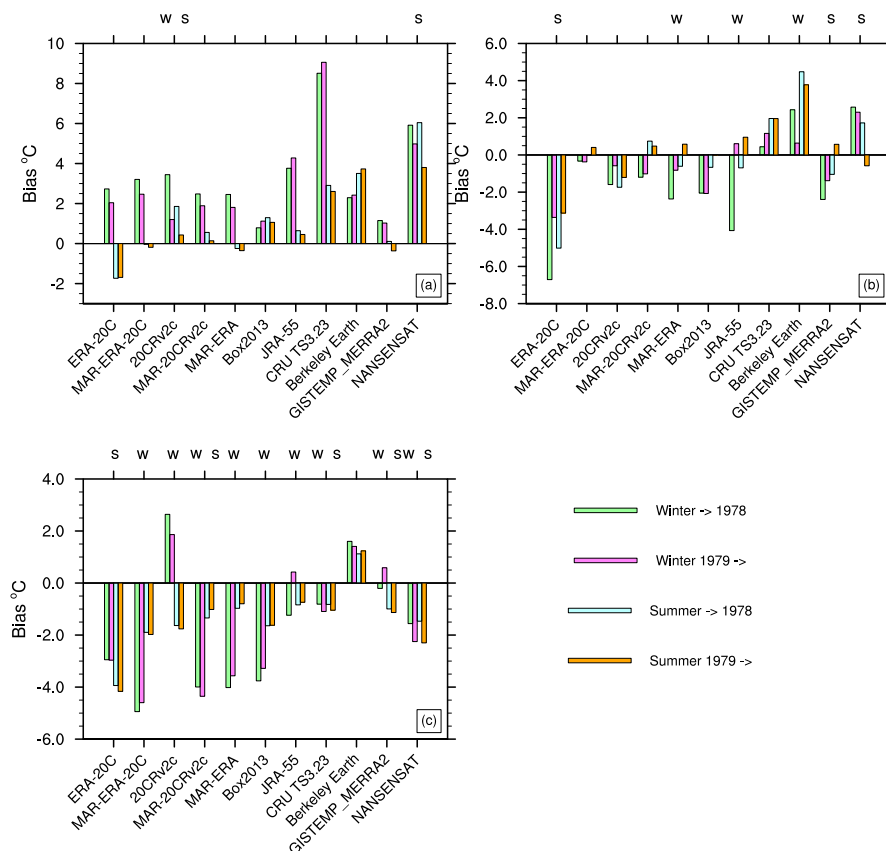
Figure 5. Monthly mean SAT bias for winter (DJF) and summer months (JJA) before and after 1979, for all datasets that extend back before 1979 (elevation-corrected where applicable) at: ice sheet stations above 1500 m (a); ice sheet stations below 1500 m (b); and coastal (DMI) stations (c). Note that these are monthly SAT biases averaged over all months in a season, not biases of seasonal mean SAT. Changes significant at the 99 % level (using Student's t test with unequal variances) are denoted by w (for winter) and s (for summer) on the top axis.
