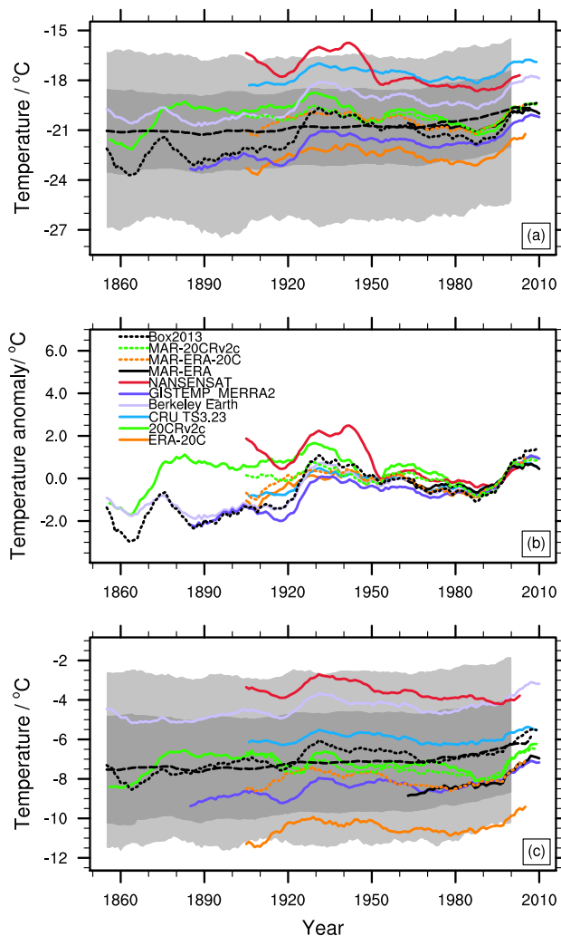
Figure 6. (a) Time series of ice sheet areal average smoothed annual mean SAT for long reanalyses, gridded temperature analyses and all three MAR variants (elevation corrected where applicable; colored lines) and CMIP5 climate models (not elevation corrected; ensemble mean in dashed black line; \pm 1 standard deviation in dark grey shading; maxima and minima in light grey shading). (b) Anomalies of ice sheet areal average smoothed annual mean SAT from long reanalyses, gridded temperature analyses and both MAR variants, relative to 1981–2010 mean. (c) As in (a) but for June–August mean SAT. In all panels, time series are smoothed using a centered, uniform-weighted 11-year window, to highlight decadal variability and aid legibility.
