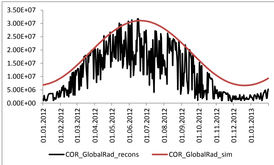
Supplementary Figure 1: Comparison of reconstructed (black) and model-estimated (red) global radiation at COR for the year 2012.
