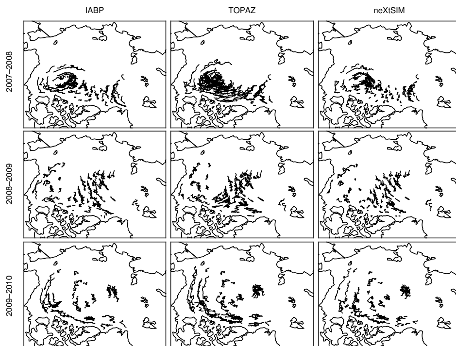
Figure 6. IABP buoys tracks (left) and their corresponding virtual tracks simulated by TOPAZ (center) and neXtSIM (right) for the winters 2007/2008 (top), 2008/2009 (middle) and 2009/2010 (bottom).
