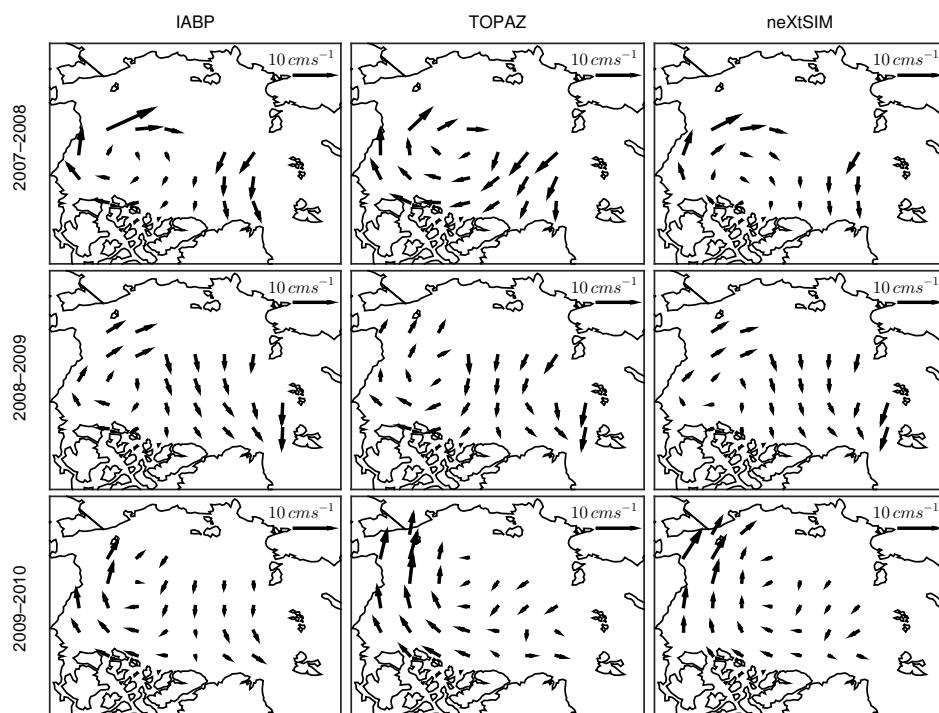
Figure 7. Mean sea-ice velocity field computed from the IABP buoys dataset (left), the corresponding float dataset generated with TOPAZ (center) and neXtSIM (right) for the winters 2007/2008 (top), 2008/2009 (middle) and 2009/2010 (bottom). The mean velocity vectors are computed with the averaging scales L = 1000 km and T = 250 days and are shown on a 400 \times 400 km regular grid.
