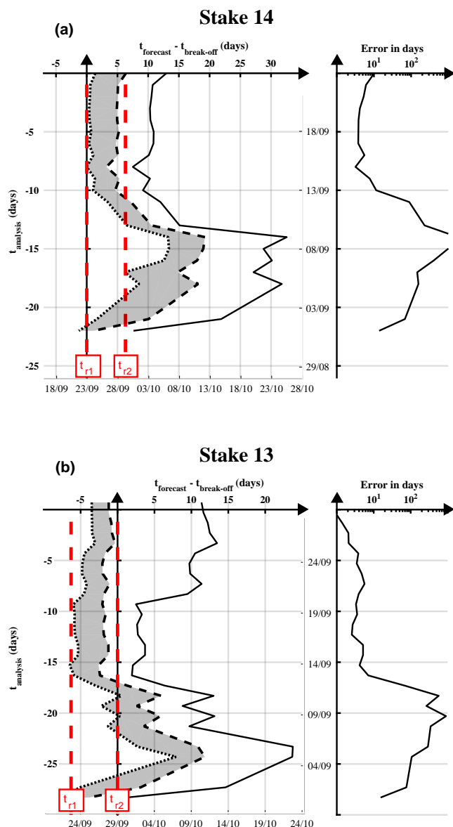
Figure 9. Evaluated critical time, t_c , for log-periodic fit (black thick line) for Stake 14 (a, left) and Stake 13 (b, left) as a function of the time of analysis using the last month of data ( t_{\text{analysis}} ). Shaded area represents the most likely break-off occurrence. This area is delimited by interrupted lines, indicating the time at which the estimated derived velocity log-periodic fit reaches 0.5 \text{ m d}^{-1} (dashed lines, v_{50} ) and 1 \text{ m d}^{-1} (dot-dash line, v_{100} ). The break-off (corresponding to 0 on horizontal axis) occurred on (a) 23 September ( t_{r1} ) and (b) 29 September ( t_{r2} ). Vertical red lines indicate the observed break-offs ( t_{r1} and t_{r2} ). Right: error in days on critical time fitted with log-periodic estimated from the 95 % confidence interval as a function of the time prior to the break-off event ( t_{\text{analysis}} ). Errors on v_{50} and v_{100} are similar to the errors on critical time, as they are directly derived from these fits.
