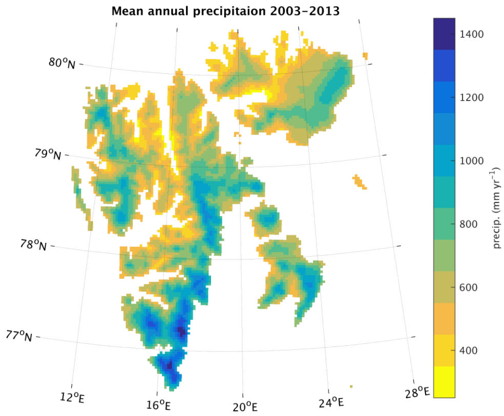
1 2 Figure S1. Mean annual precipitation (mm yr -1 ) simulated with WRF-CMB from 2003 to 3 2013. 4
