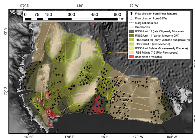
Figure 10. Control of sea floor geology on ice dynamics. Geologic boundaries were interpolated from legacy seismic lines (shown here) with pre-interpreted seismic units by Anderson and Bartek (1992) and Brancolini et al. (1995). The WRS is characterized by complex, older, and more consolidated strata, where ice streams have eroded down to Oligocene-age strata. Volcanic islands and seamounts outcrop in the southern portion of the WRS. The western side of Glomar Challenger Basin, bordering Ross Bank, contains older and more variable geologic strata outcropping at the sea floor, including a patch of basement outcrop on the inner shelf. In general, thick unconsolidated Plio-Pleistocene strata fill most of the ERS and increase in thickness in an offshore direction (Alonso et al., 1992). Plio-Pleistocene sediments are thin in southern Whales Deep, overlying older Miocene strata. Eastern Little America Basin is characterized by lithified late Oligocene through Miocene deposits. Arrows indicating flow direction are based on geomorphic features.
