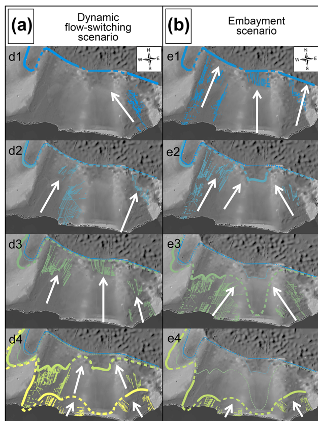
Figure 8. Possible retreat scenarios for the eastern Ross Sea interpreted from flow sets. (a) The dynamic flow-switching scenario calls for alternating regional flow directions, followed by north–south recession of the grounding line. This model requires preservation of at least three different flow fabrics as ice remains grounded on the outer continental shelf. (b) In the embayment scenario, a large grounding-line embayment in the eastern Ross Sea forms over Whales Deep. The embayment scenario is independently more consistent with inland palaeo-ice thickness reconstructions and sea floor seismic observations.
