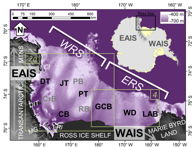
Figure 1. Regional bathymetry of the Ross Sea continental shelf with bed topography data acquired from BEDMAP2 (Fretwell et al., 2013). Inset shows the West and East Antarctic ice sheets (WAIS and EAIS), separated by the Transantarctic Mountains with the Ross Sea study area outlined. Locations for Fig. 2a and Fig. 4 are shown. WRS (Western Ross Sea), ERS (Eastern Ross Sea), EAIS (East Antarctic ice sheet), WAIS (West Antarctic ice sheet), DT (Drygalski Trough), JT (JOIDES Trough), PT (Pennell Trough), CB (Central Basin), CrB (Crary Bank), PB (Pennell Bank), RB (Ross Bank), GCB (Glomar Challenger Basin), WD (Whales Deep), LAB (Little America Basin), CI (Coulman Island), DIT (Drygalski Ice Tongue), MG (Mackay Glacier), MS (McMurdo Sound).
